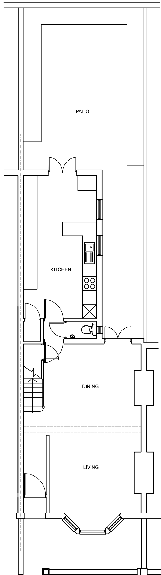
EXISTING GROUND FLOOR PLAN + SITE PLAN
