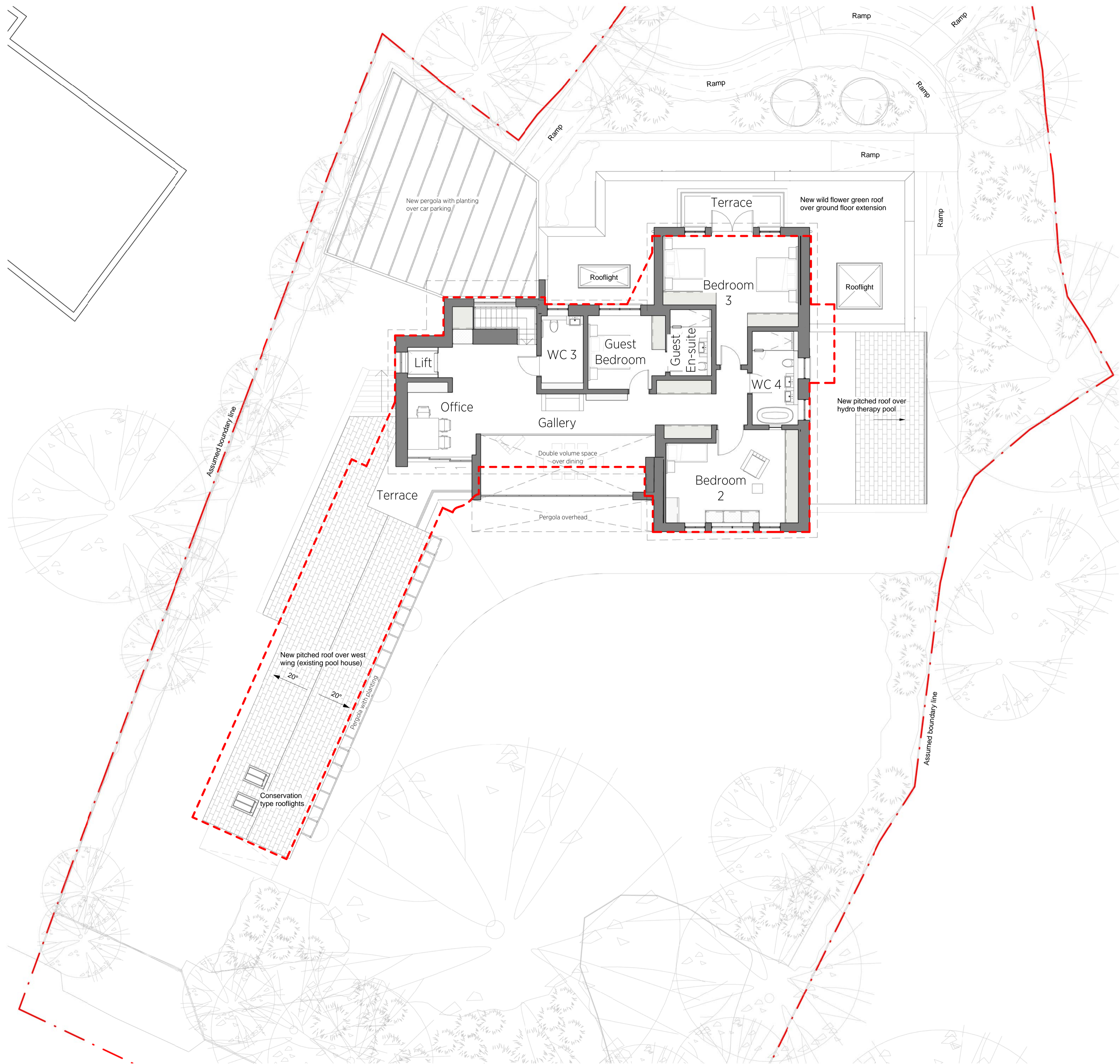
1 Proposed First Floor 1:100 @ A1
