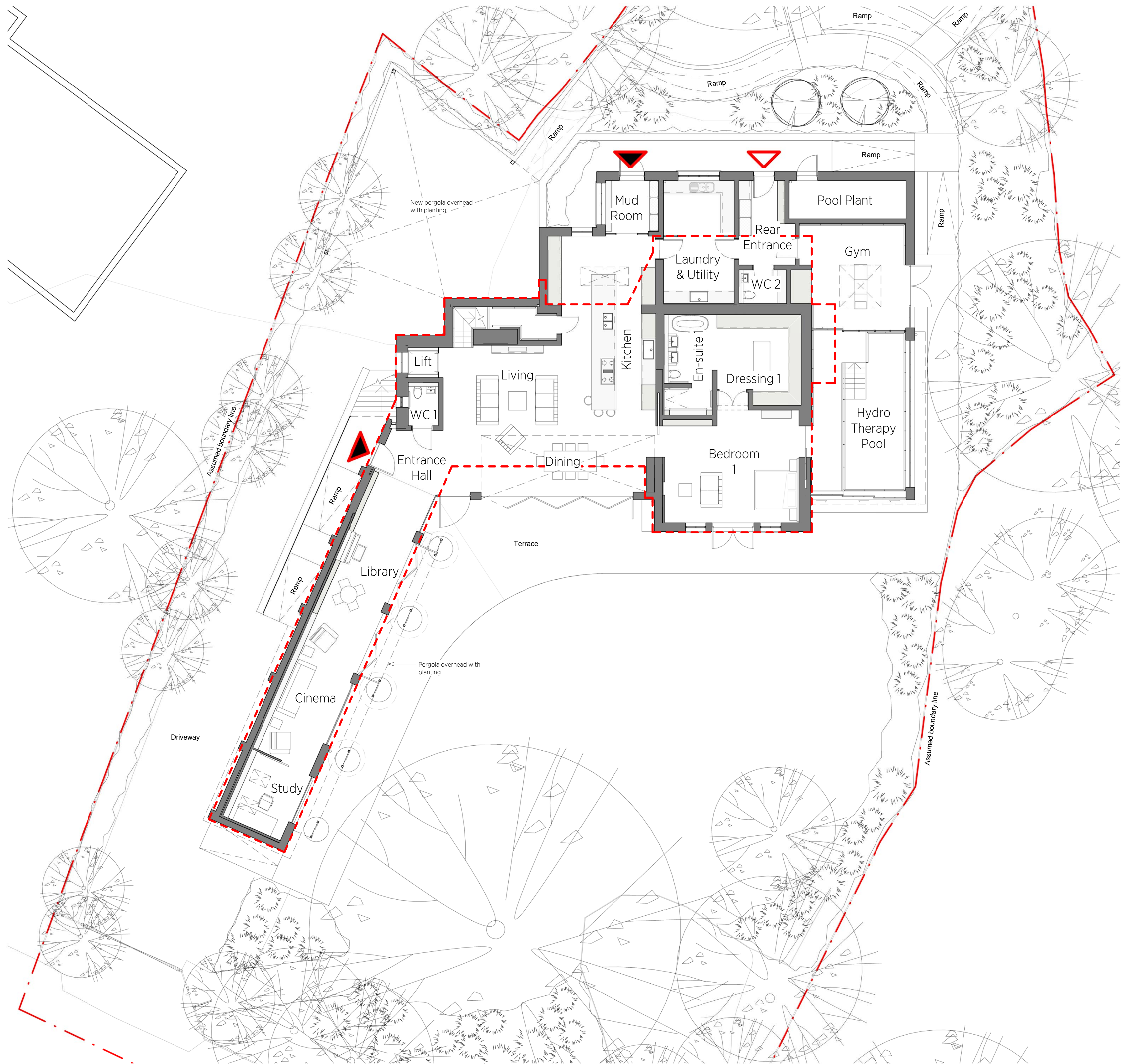
1 Proposed Ground Floor 1:100 @ A1
