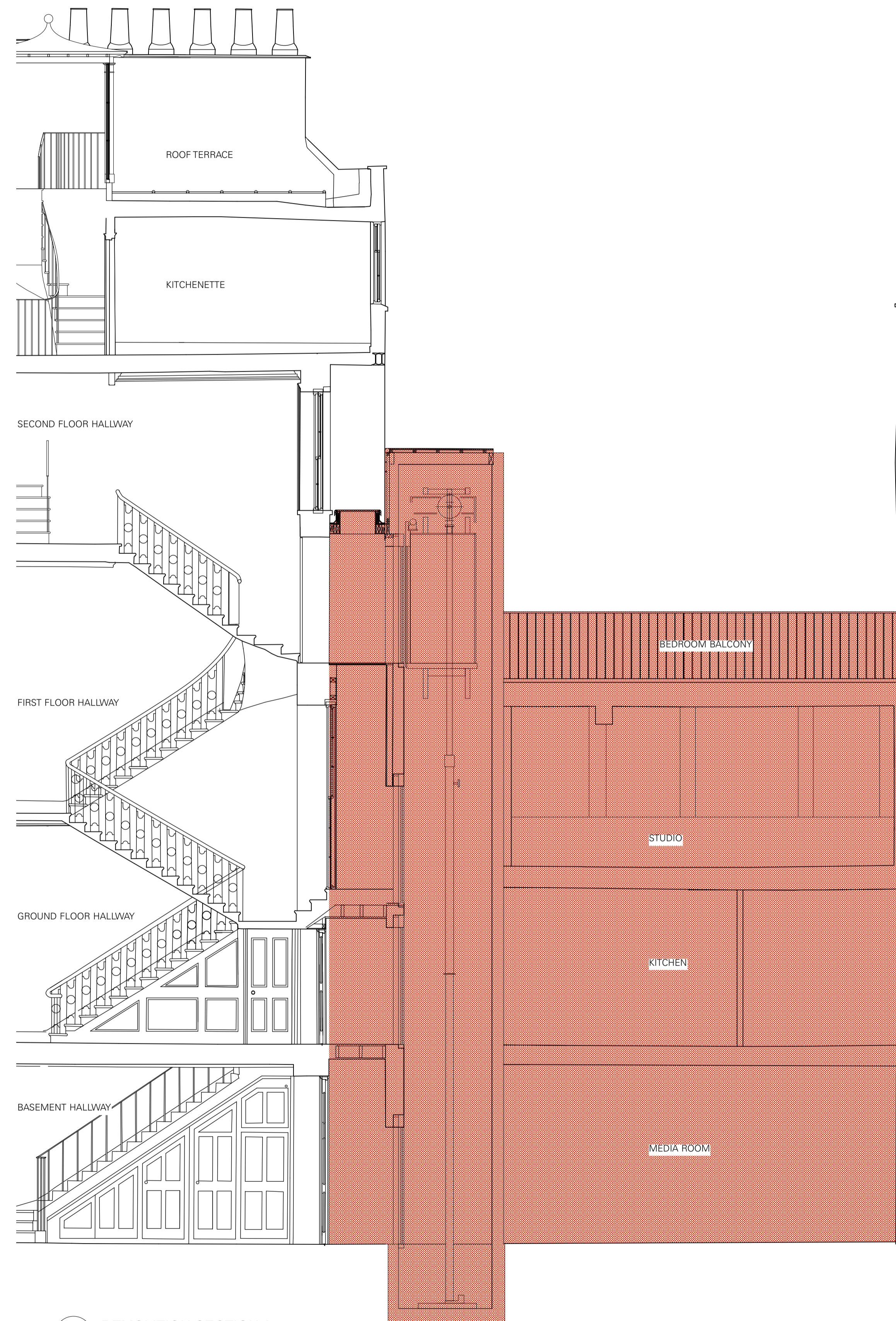
DEMOLITION SECTION A 1:50 @ A1, 1:100 @ A3
