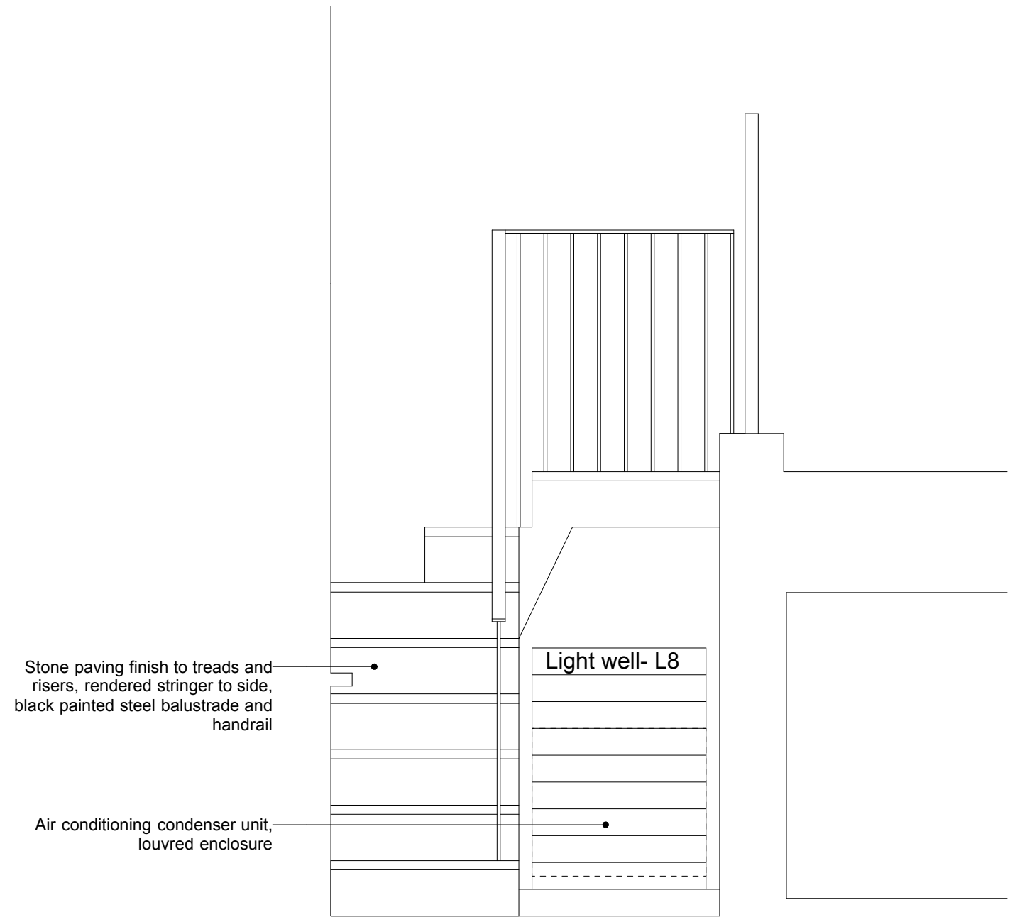
Stair Elevation
