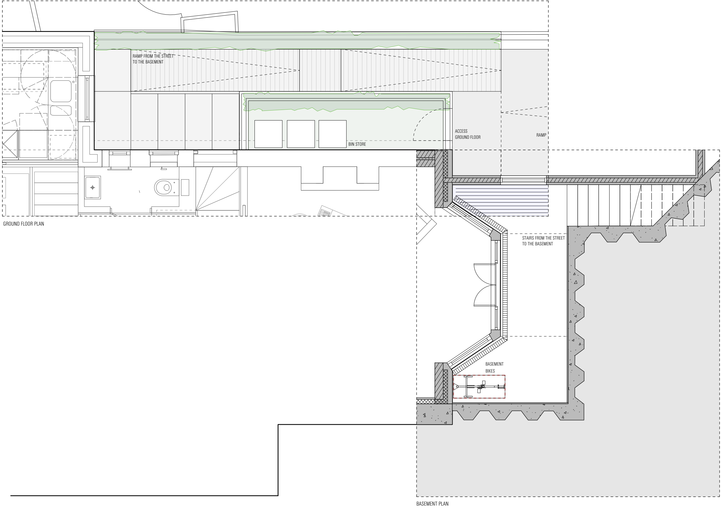
BASEMENT PLAN
