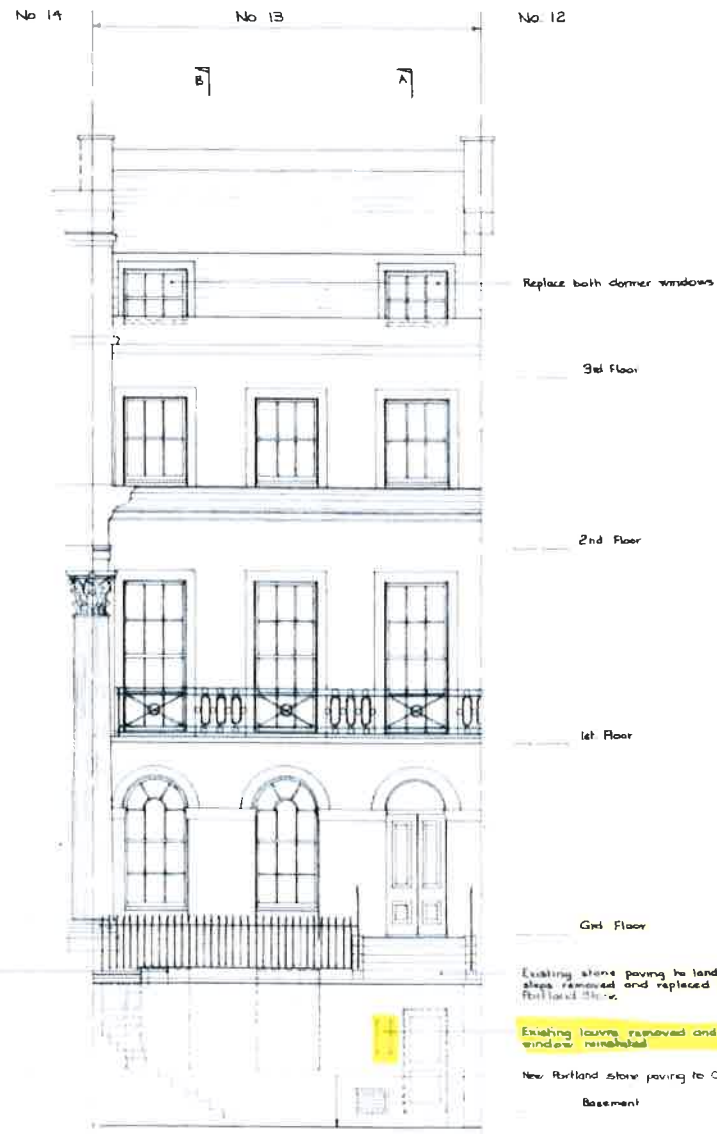
AS PROPOSED FRONT ELEVATION
