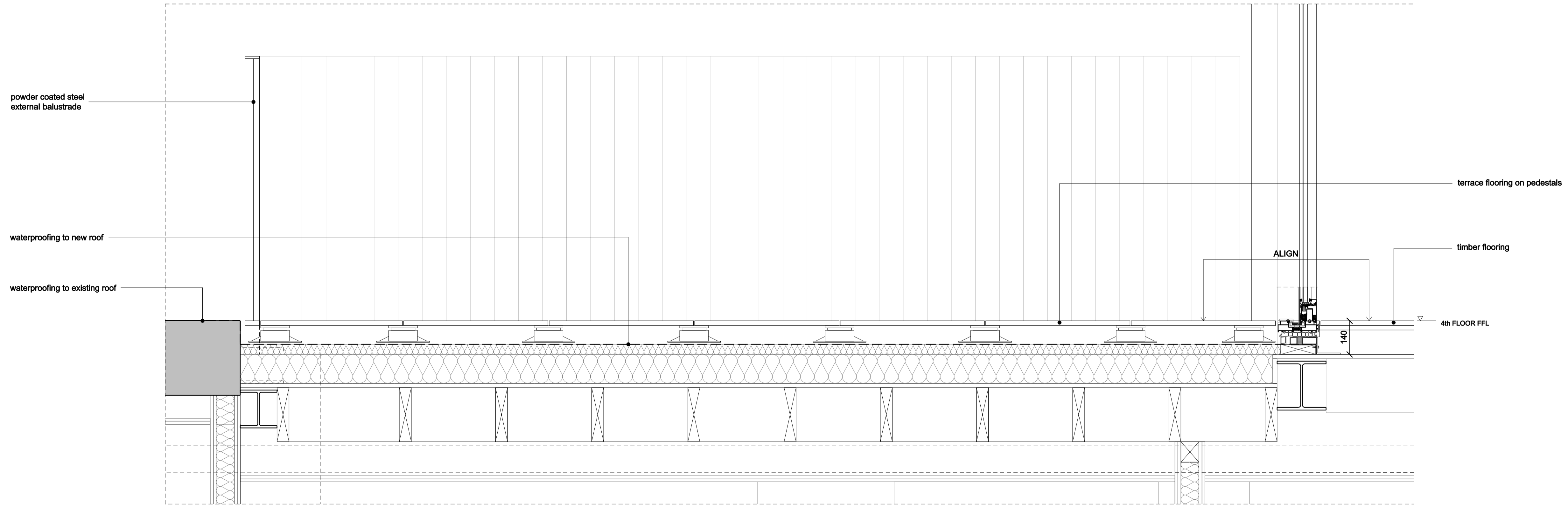
02. 4th FLOOR TERRACE LONG SECTION
