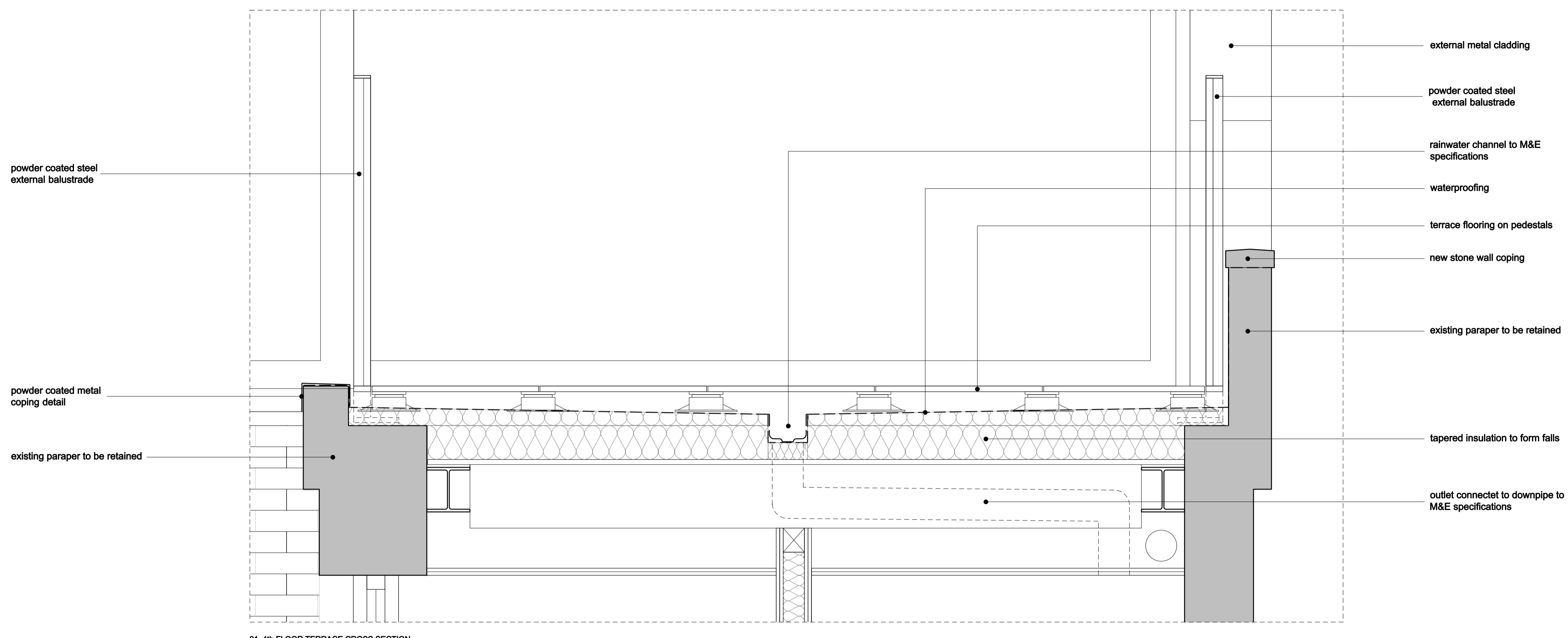
01. 4th FLOOR TERRACE CROSS SECTION
