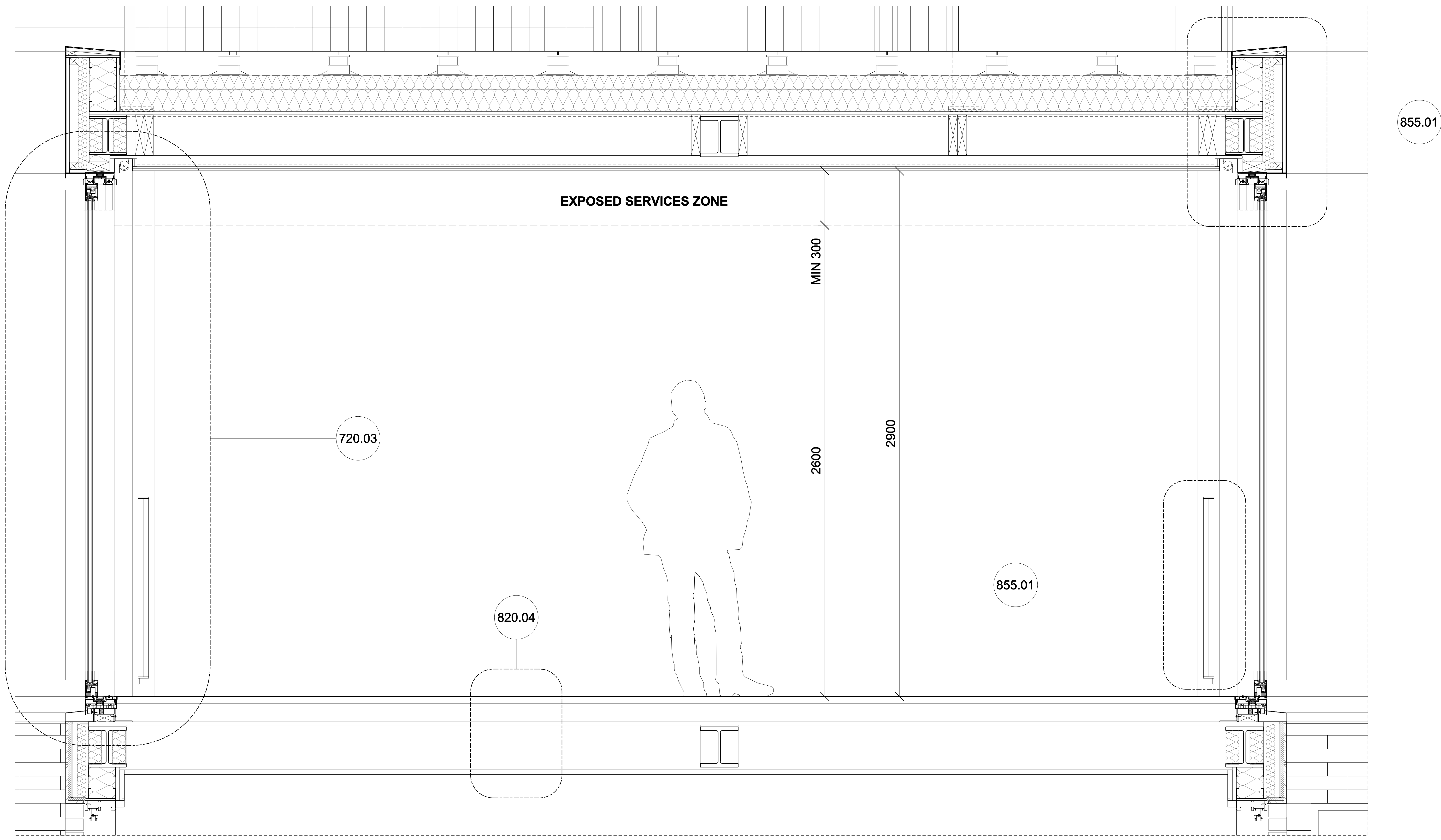
01. 4TH FLOOR OFFICE CROSS-SECTION THROUGH GLAZING
