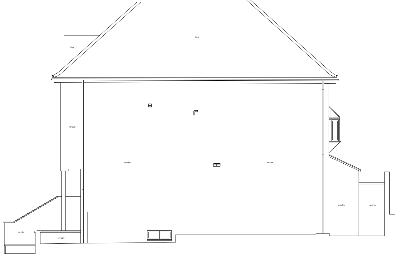
Proposed side / east elevation
