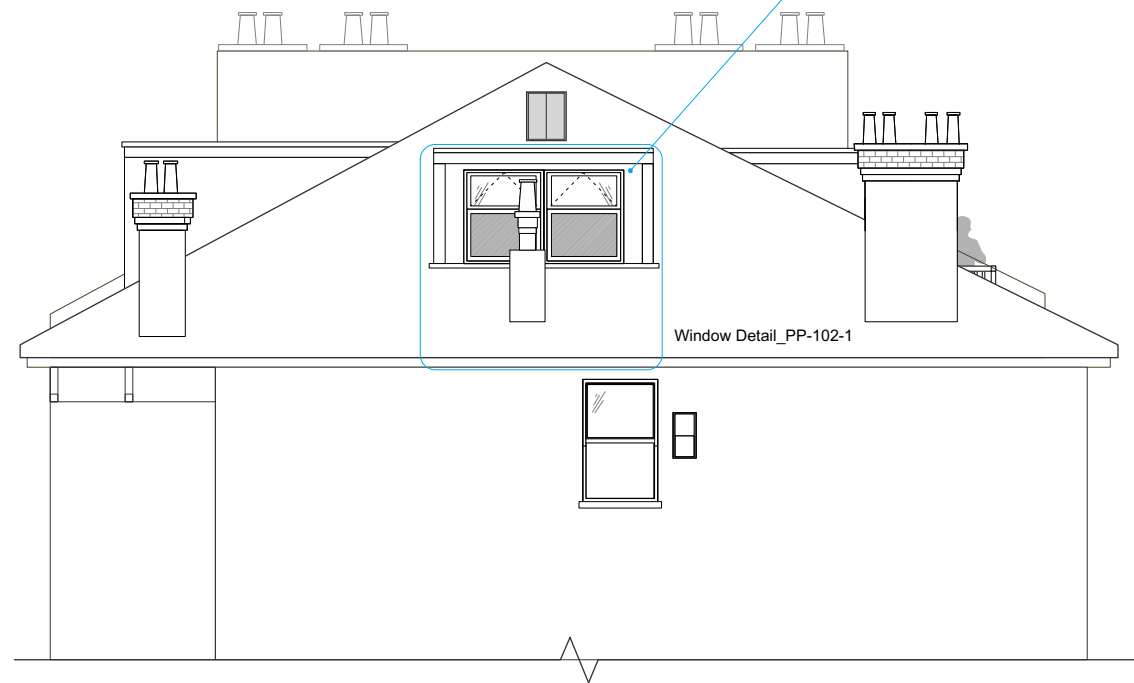
62 BELSIZE PARK- PROPOSED SIDE ELEVATION Scale: 1:100
