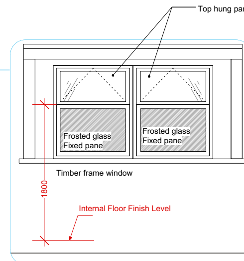
Window Detail_PP-102-1 Scale: 1:50
