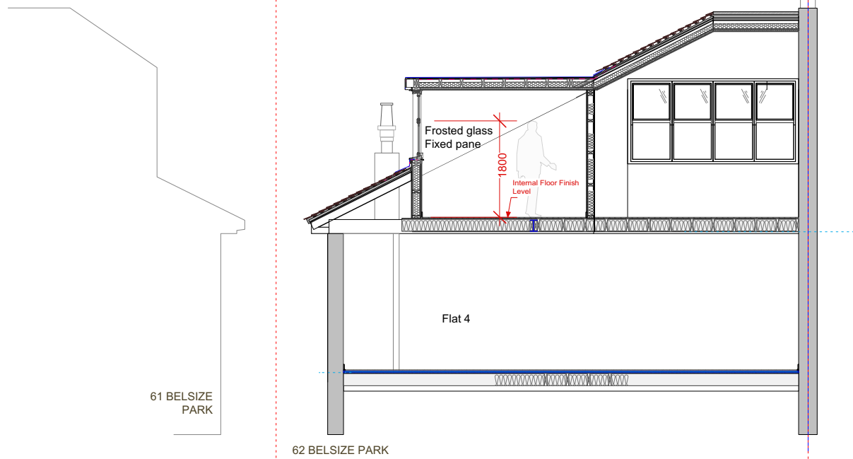
62 BELSIZE PARK- PROPOSED SECTION BB Scale: 1:100
