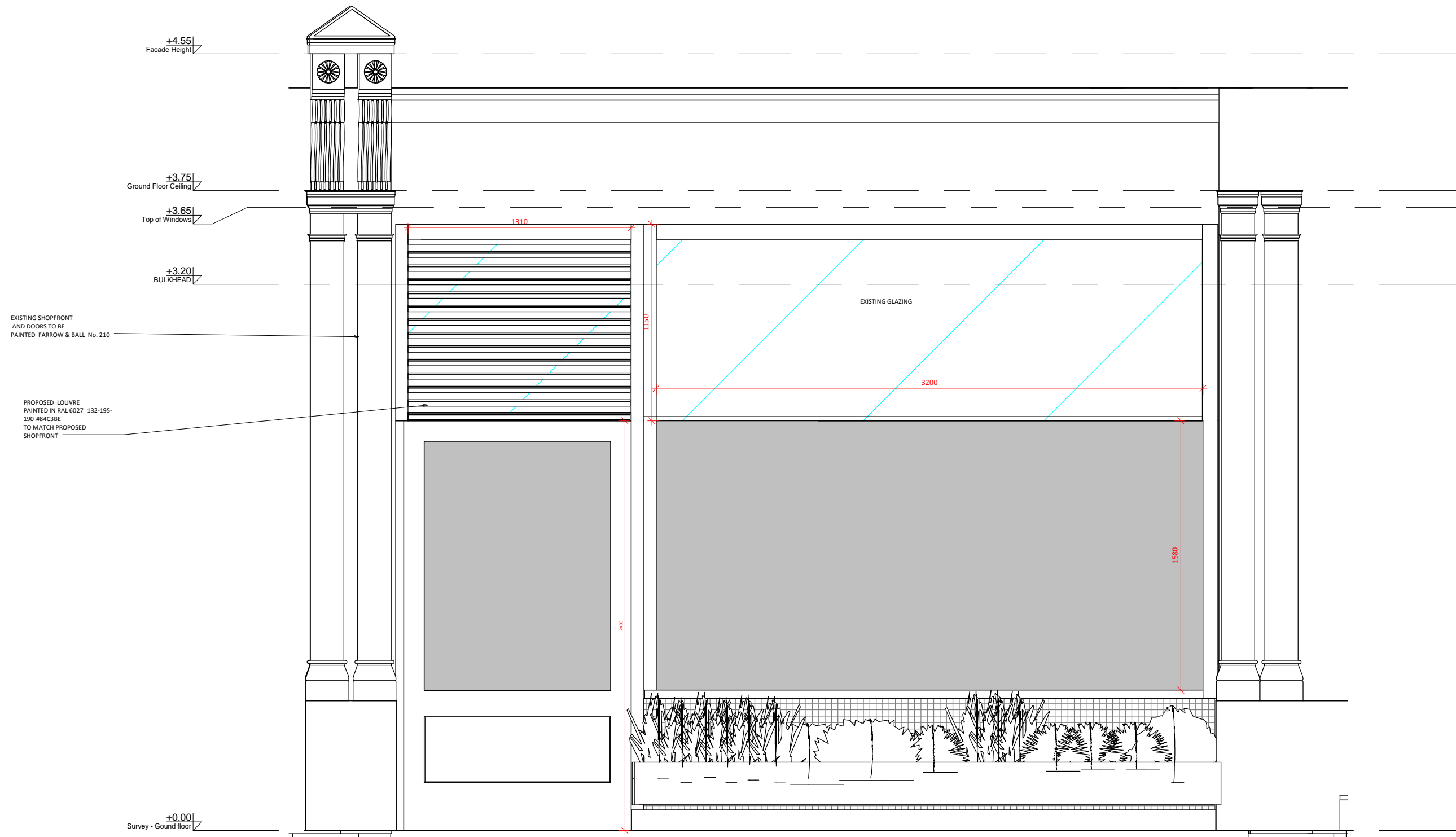
1 Proposed -Louvre 1:25
