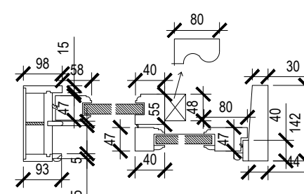
Sash Window On Weights- SIDE VIEW
