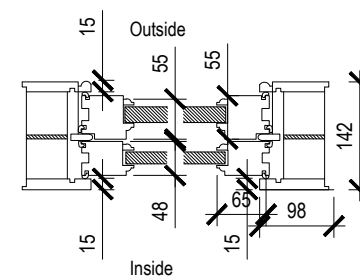
Sash Window On Weights- TOP VIEW
