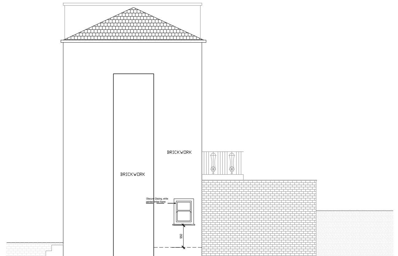
Side Elevation
