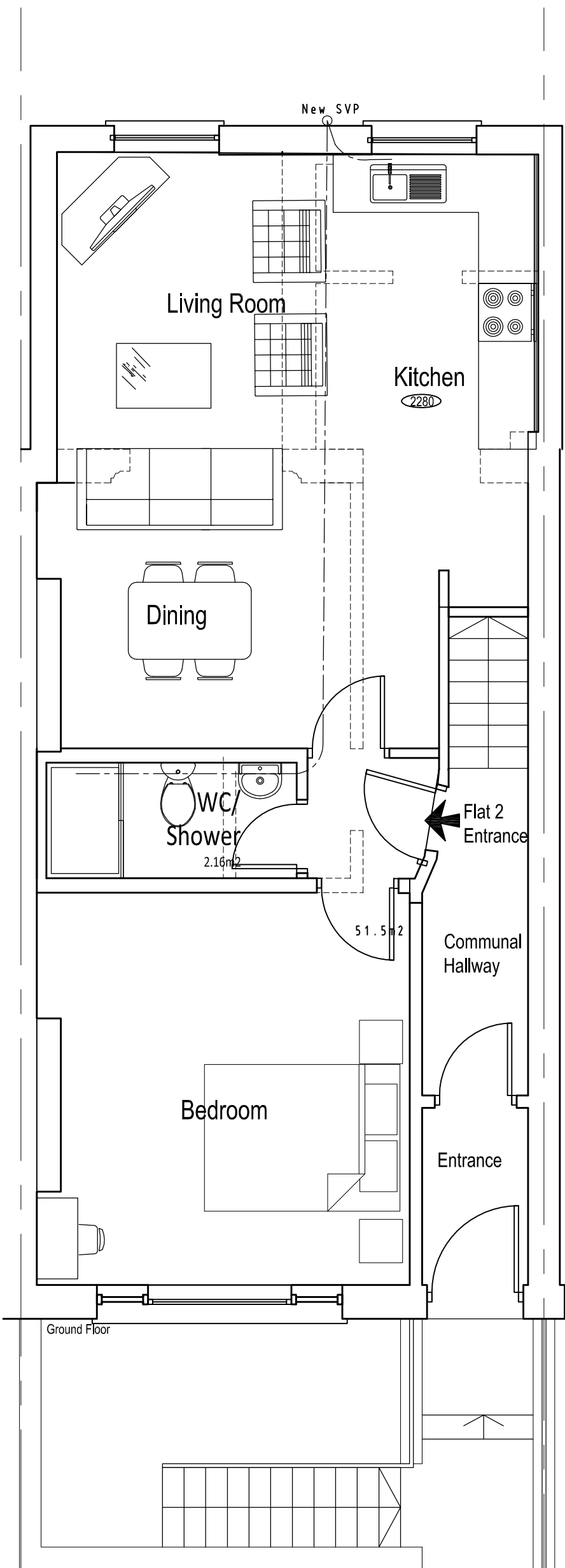
7A PROPOSED GROUND FLOOR PLAN SCALE 1:50
