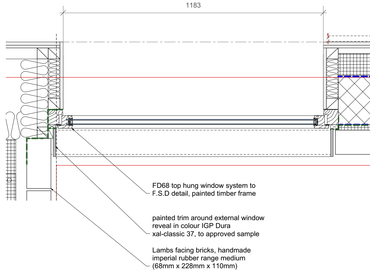
1 basement lightwell window_plan Scale: 1:10
