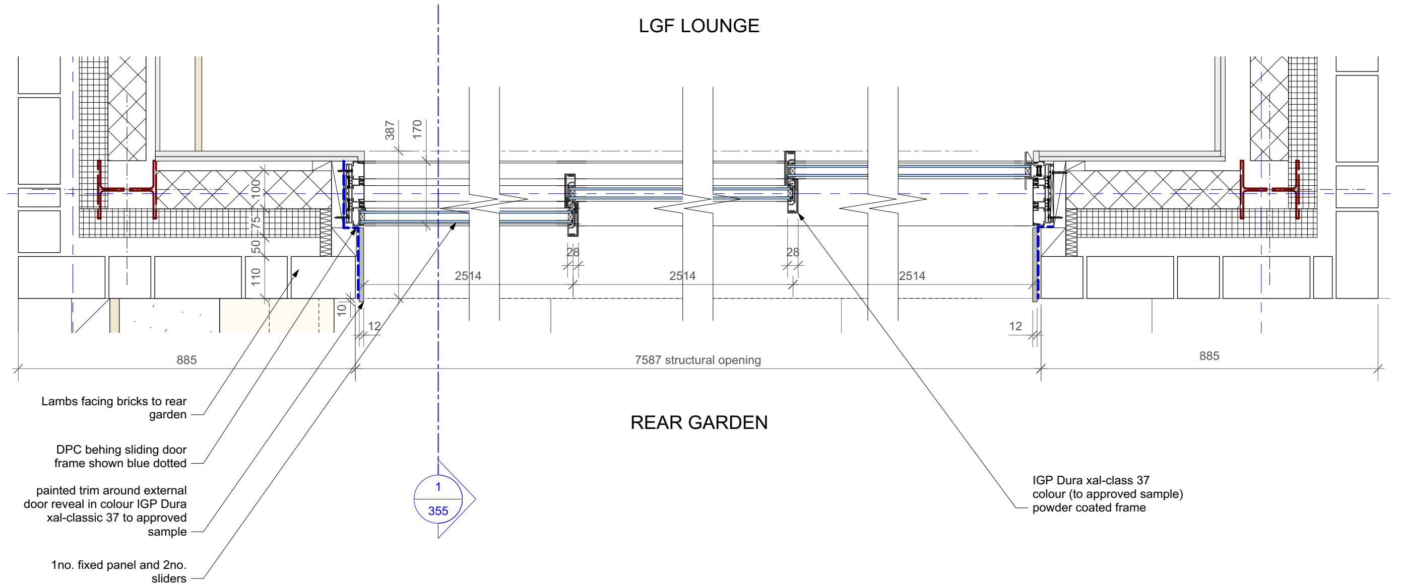
1 rear sliding door_plan Scale: 1:10
