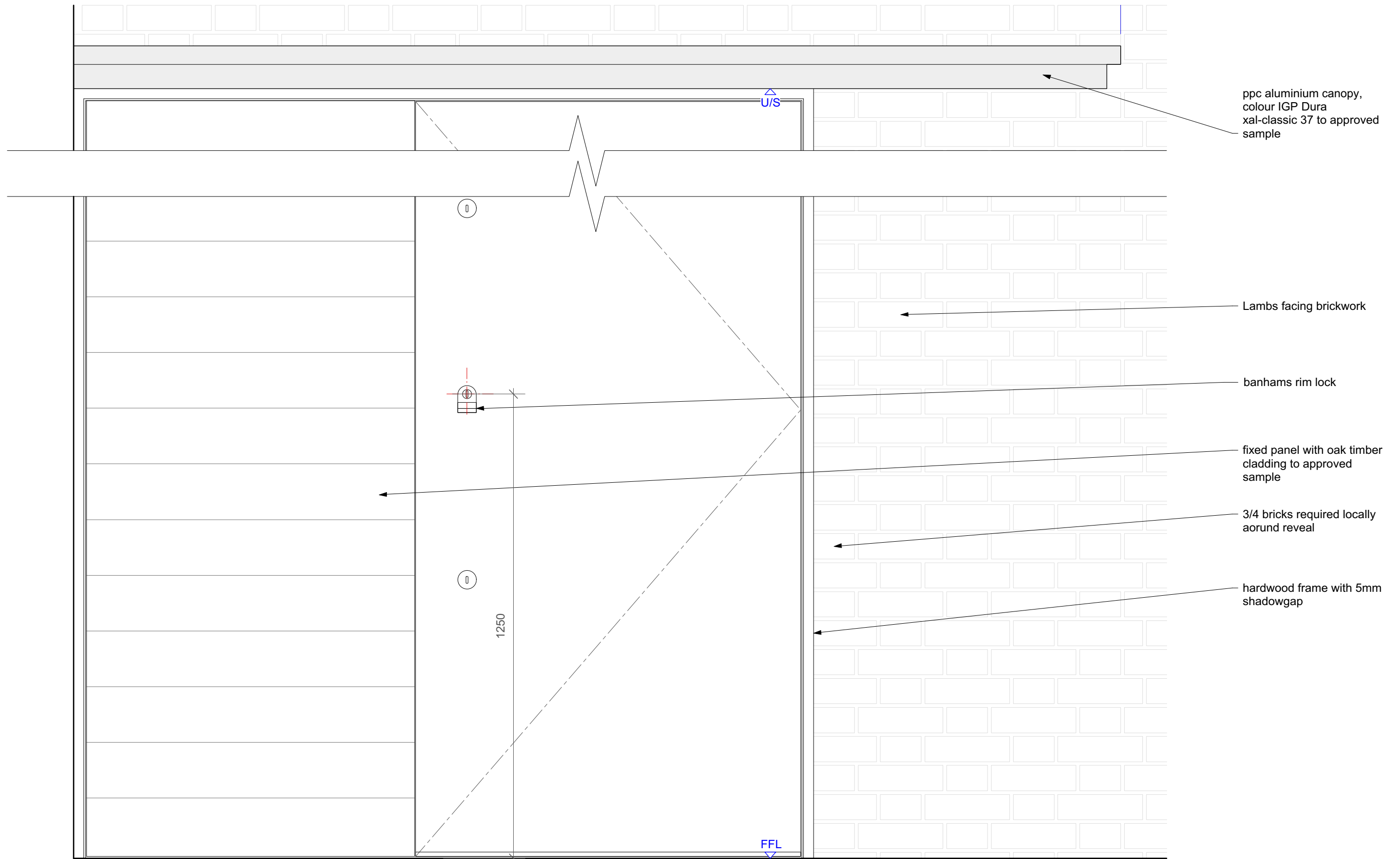
1 front door external elevation Scale: 1:10
