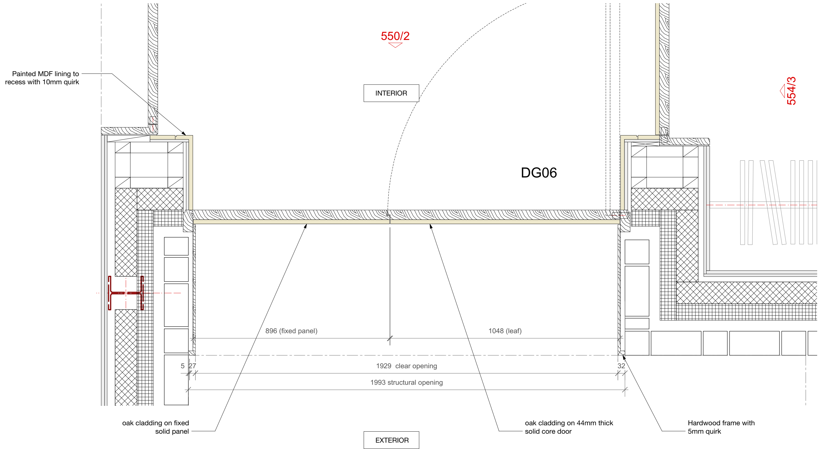
1 front door_plan Scale: 1:10
