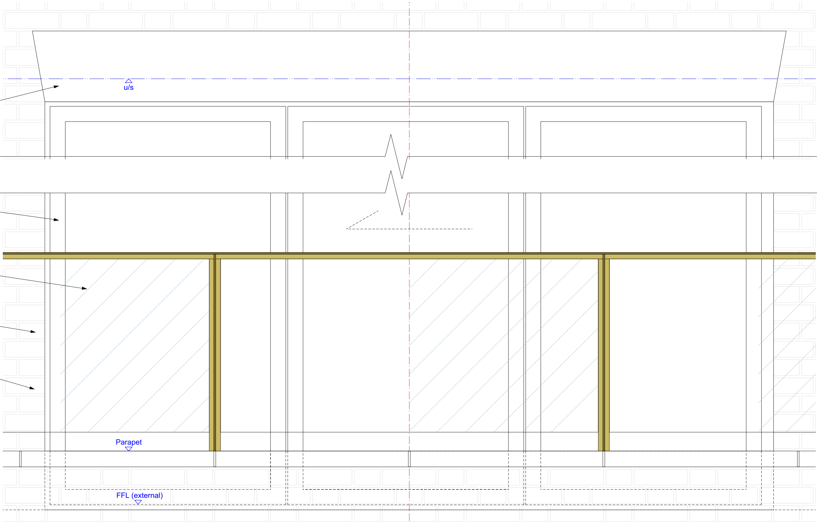
1 rear folding sliding doors_external elevation Scale: 1:10
