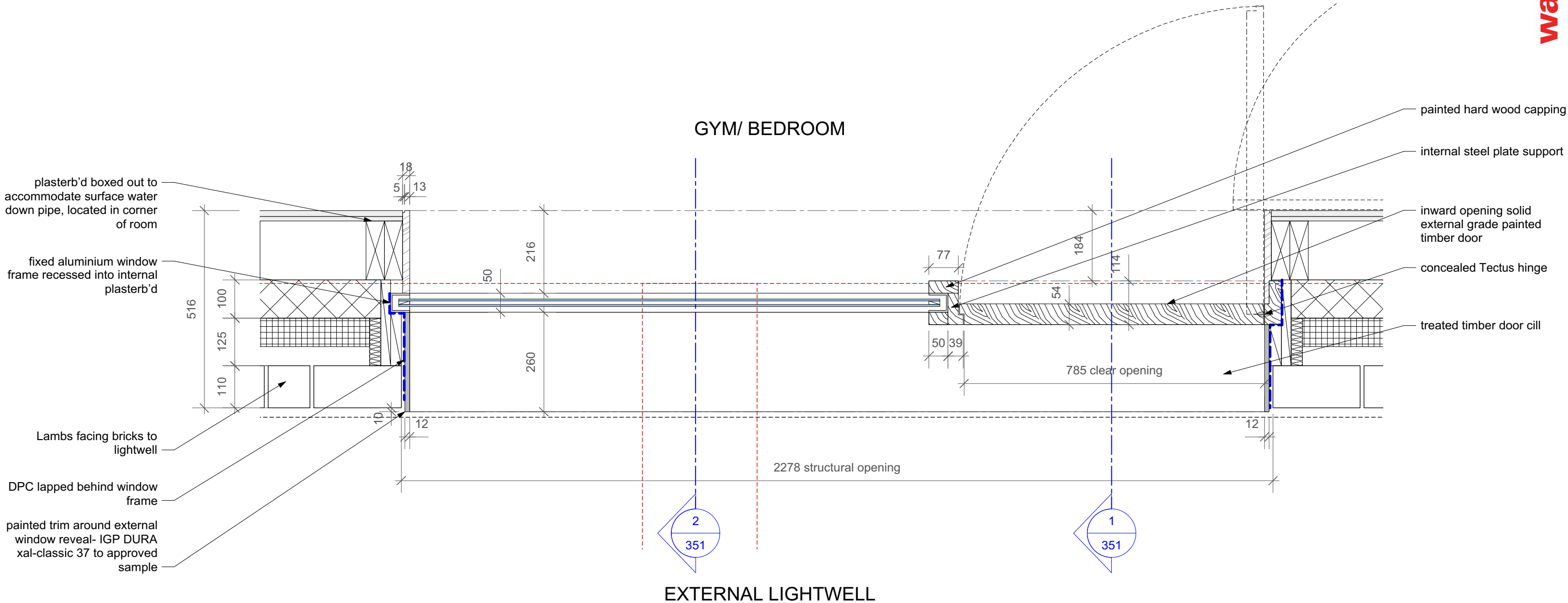
1 lightwell door_plan Scale: 1:10
