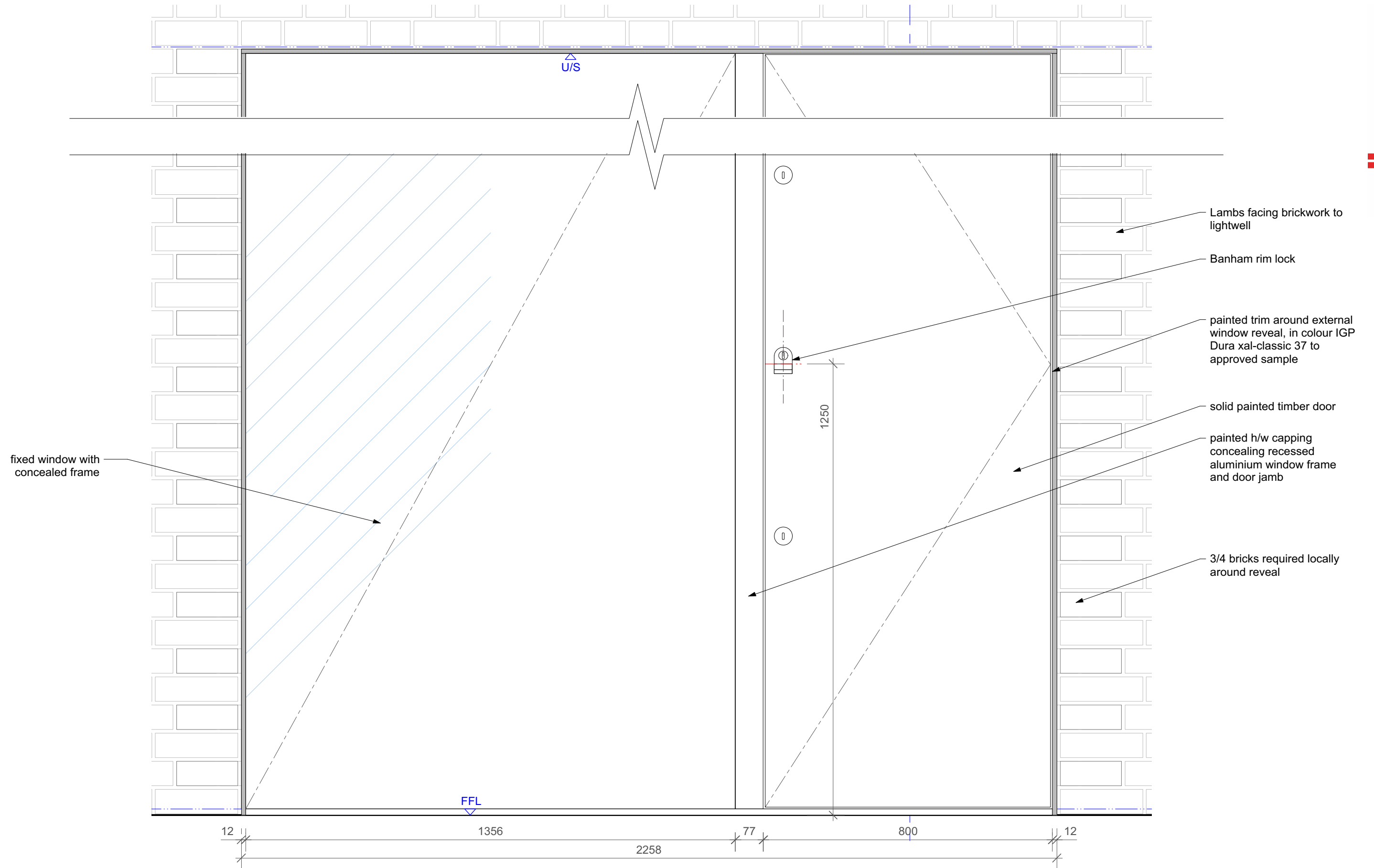
1 lightwell door_external elevation Scale: 1:10
