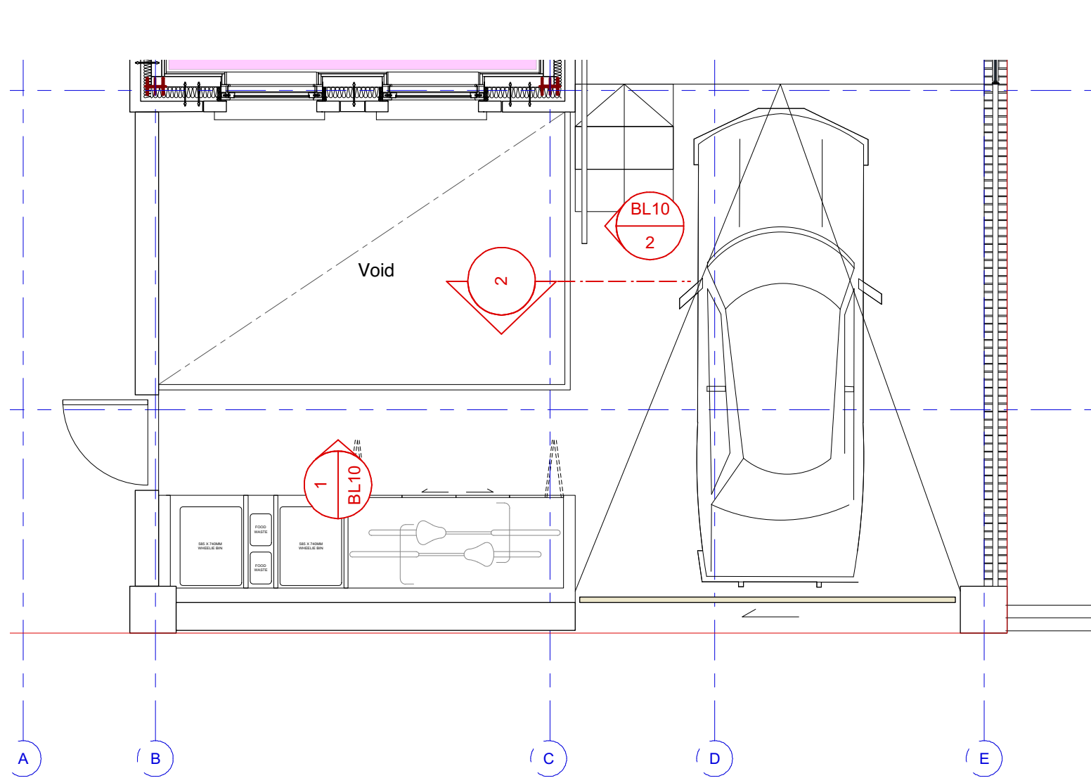
1 GF drive and lightwell_plan Scale: 1:50
