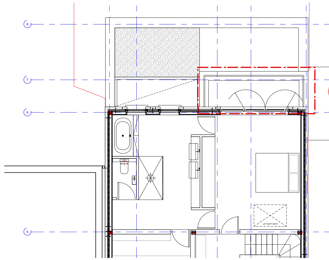
2 balustrades_FF reference plan Scale: 1:100
