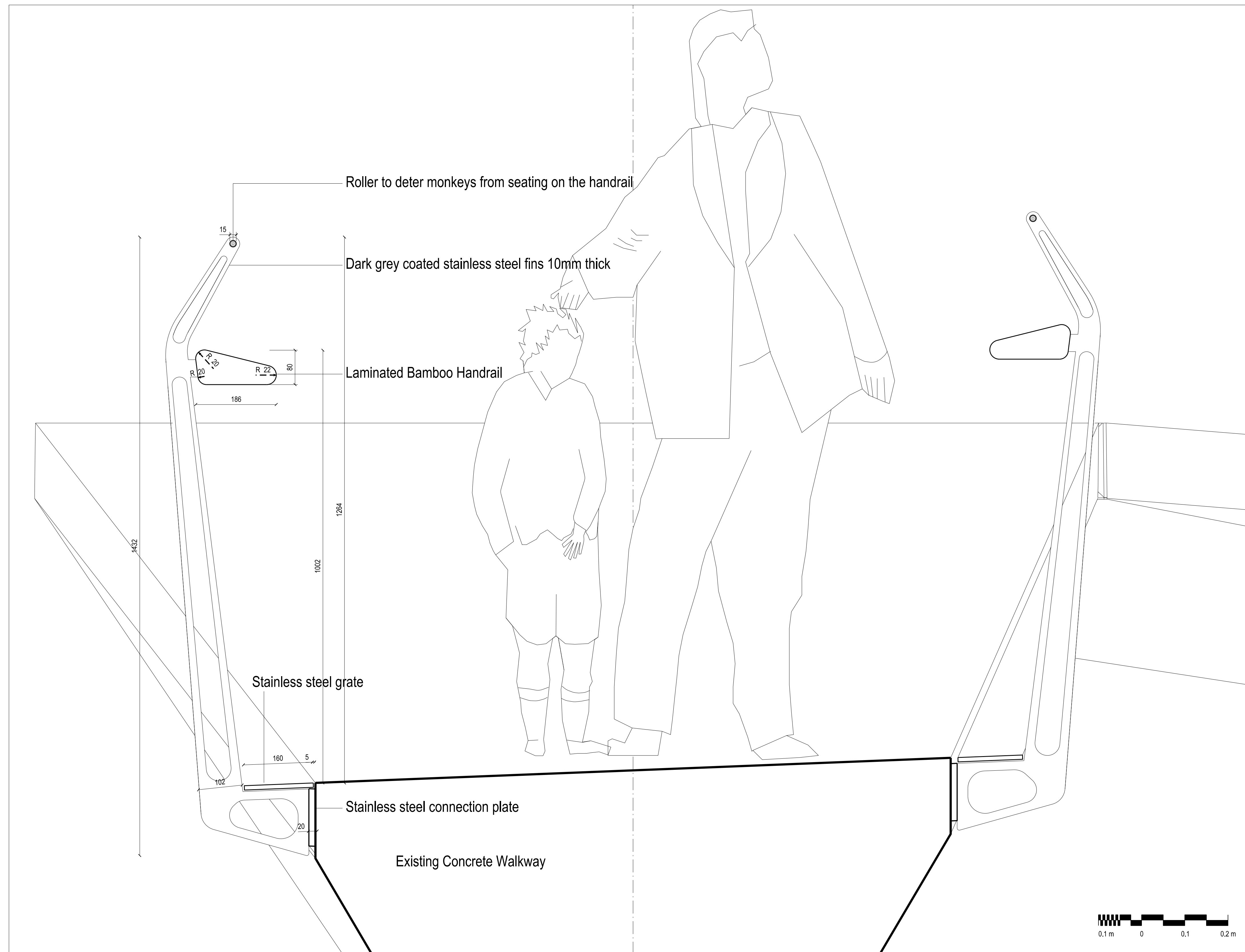
01 Walkway Balustrade Detail
