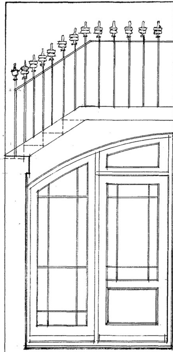
1:20 SCALE ENCLOSURE - ENTRANCE SCREEN TO PAVEMENT UTILITY ROOM.
