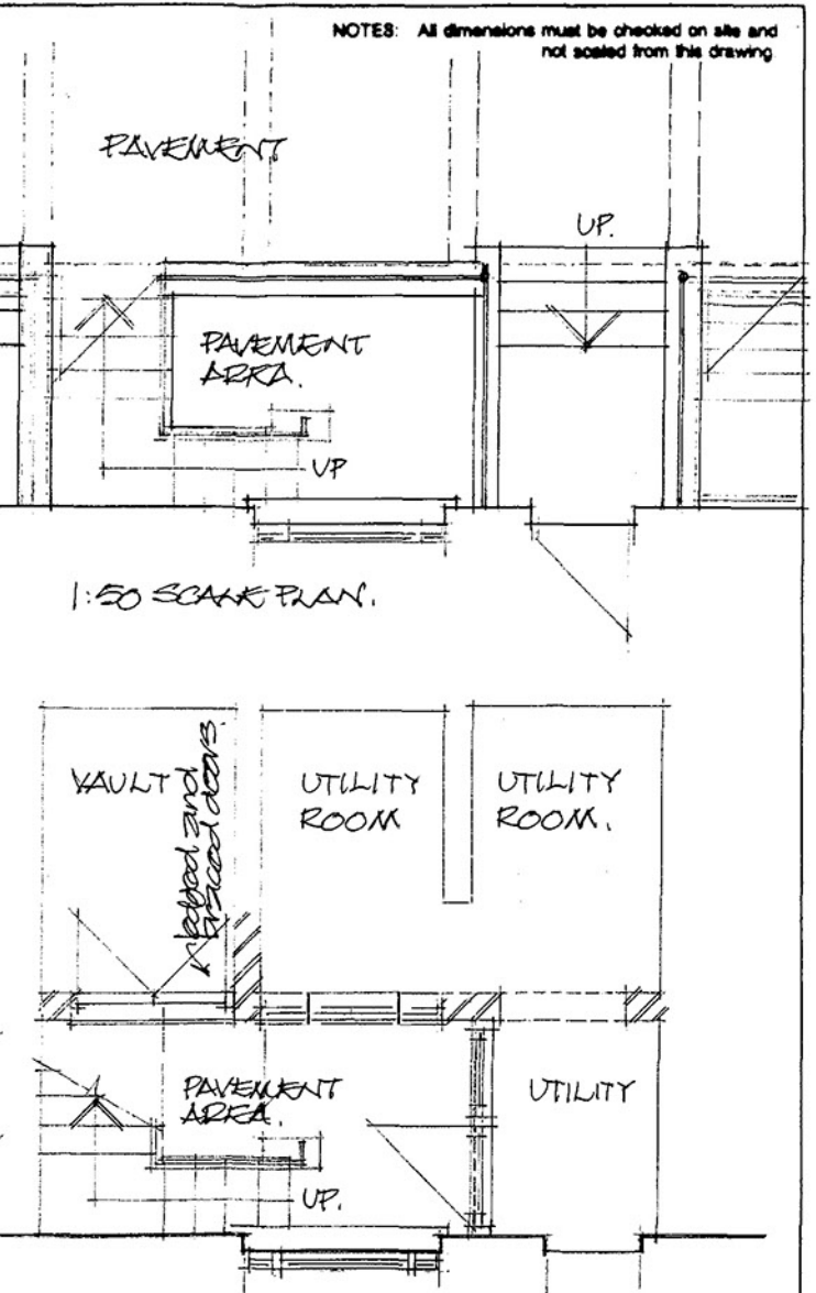
1:50 SCALE PLAN VAULTS AND UTILITY ROOM.
