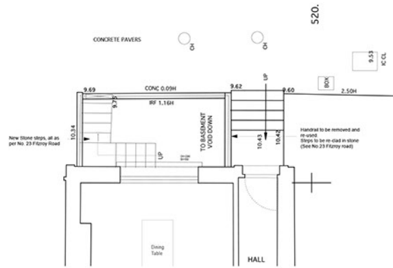
PART PLAN (UPPER GROUND)
