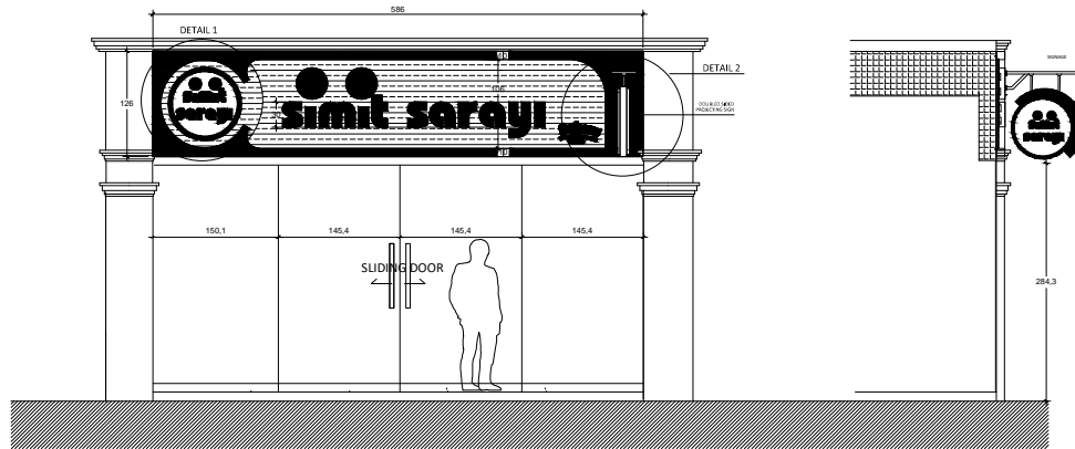
PROPOSED ELEVATION-SECTION
