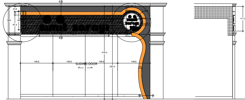
AS BUILT ELEVATION-SECTION
