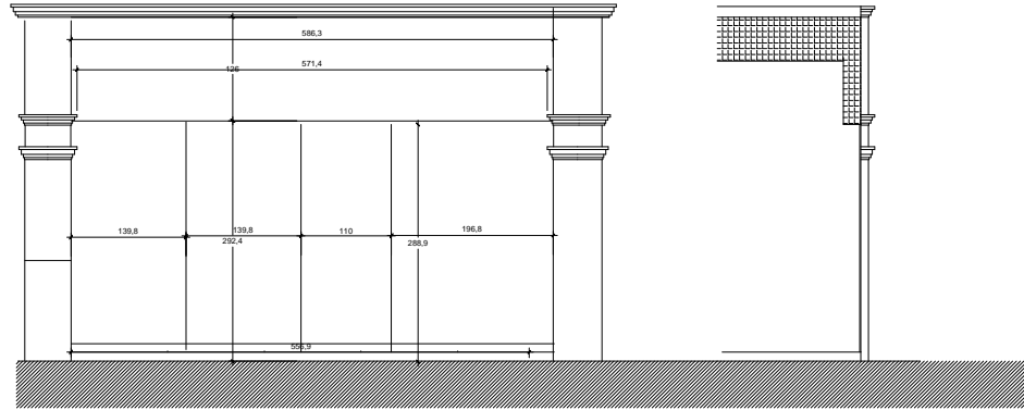
PRE-BUILT ELEVATION-SECTION
