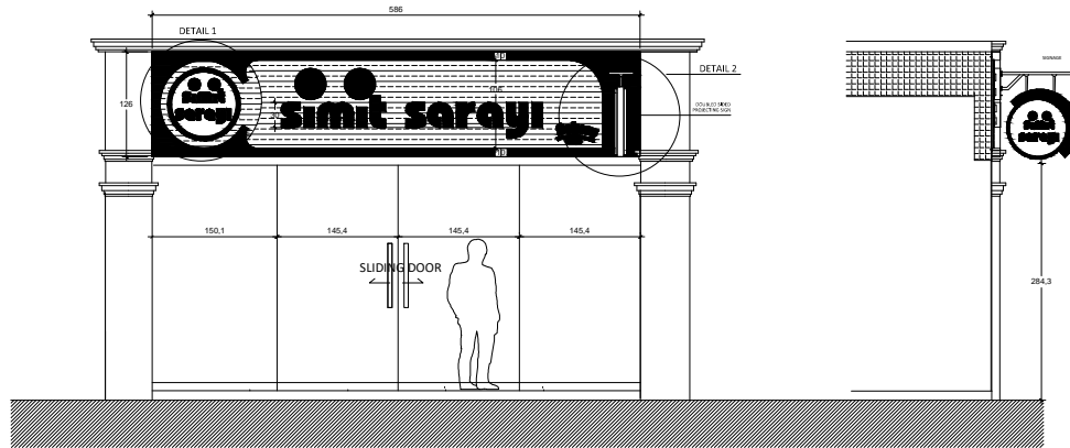
PROPOSED SHOPFRONT ELEVATION
