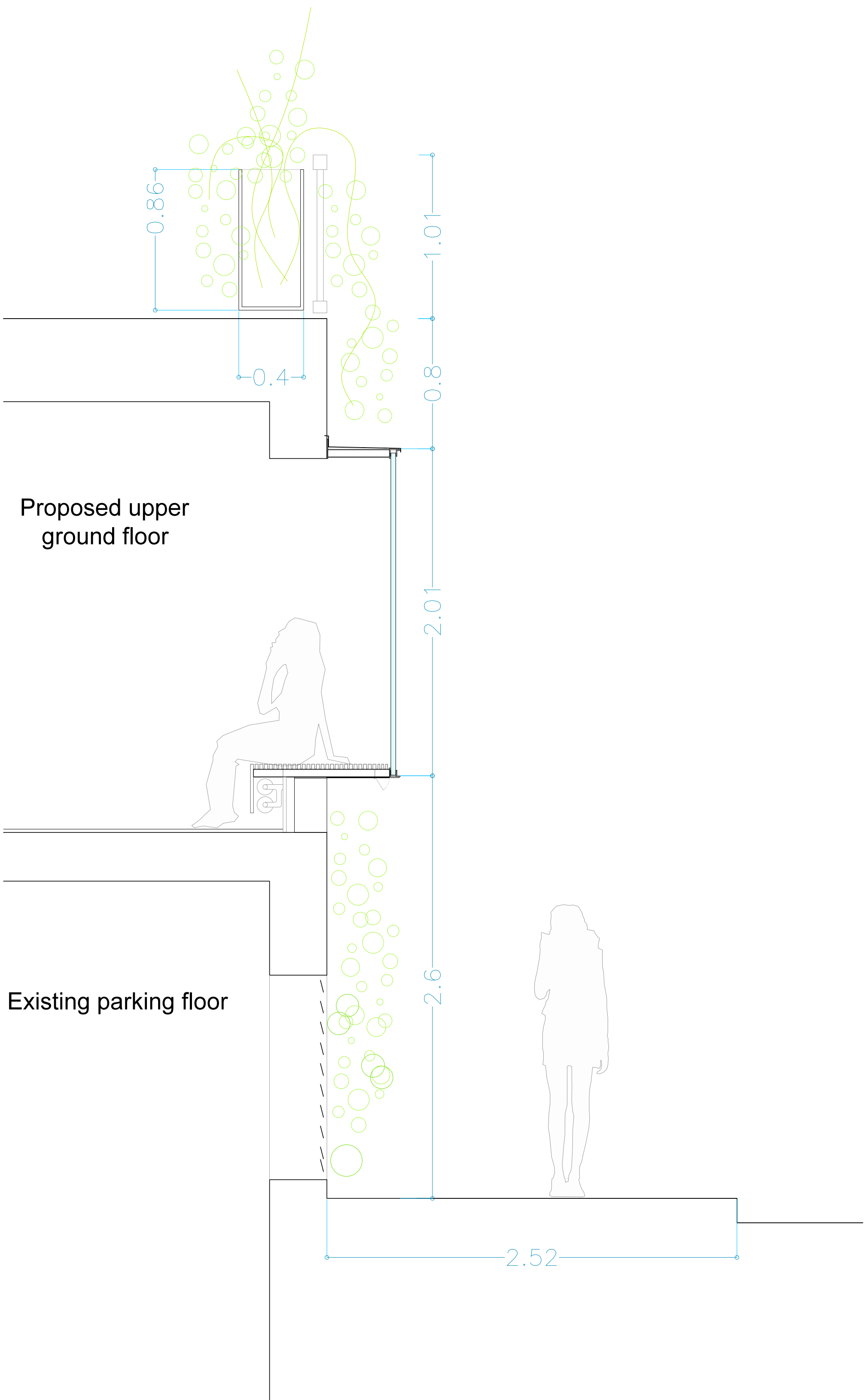
PROPOSED DETAILED SECTION AA sc 1:20
