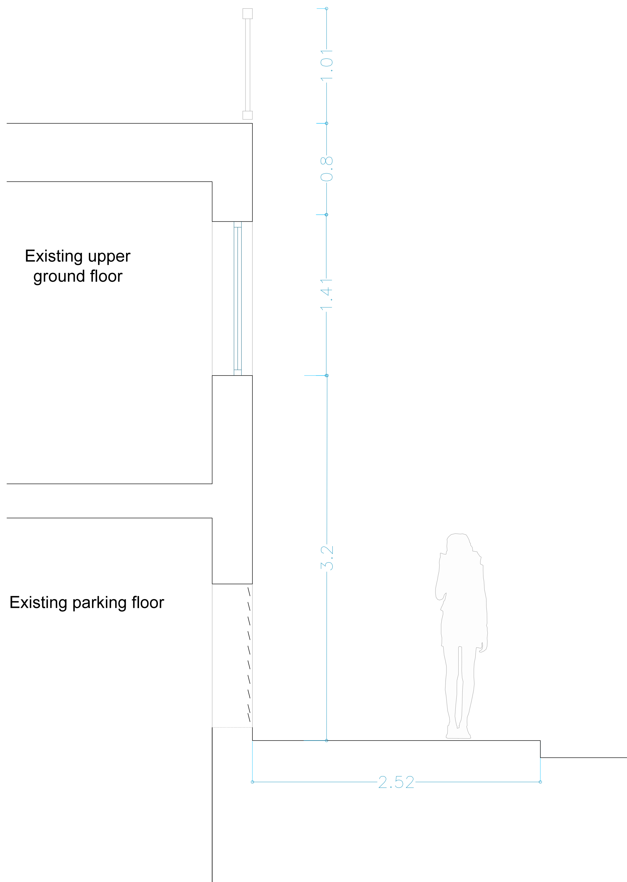
EXISTING DETAILED SECTION AA sc 1:20
