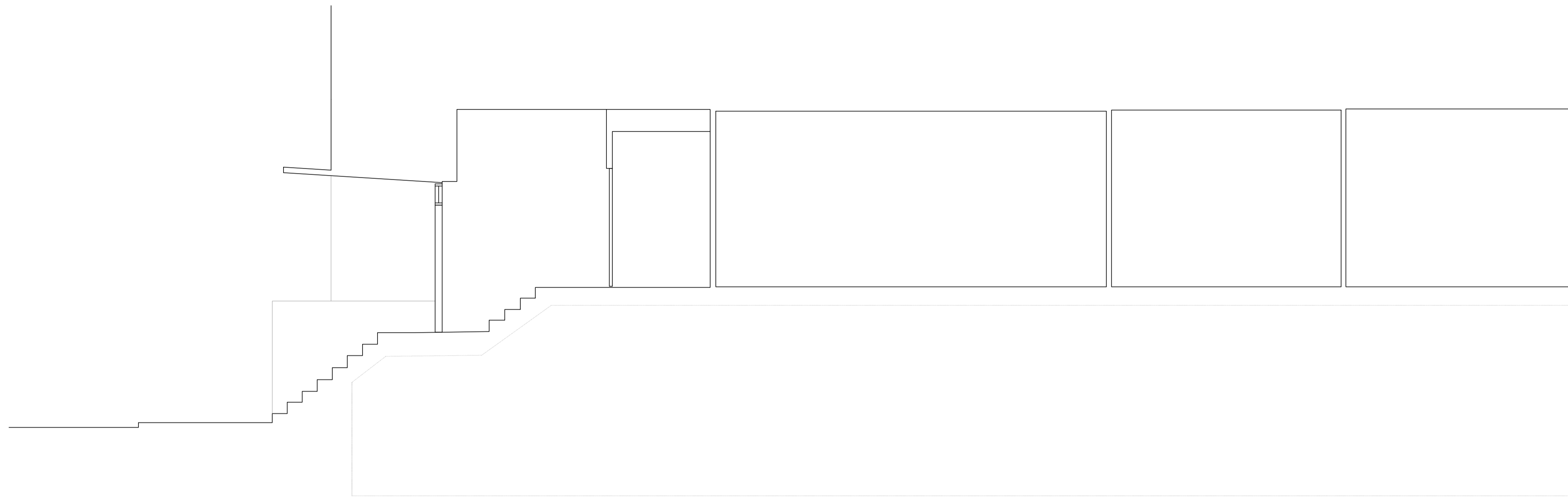
EXISTING SECTION BB sc 1:50
