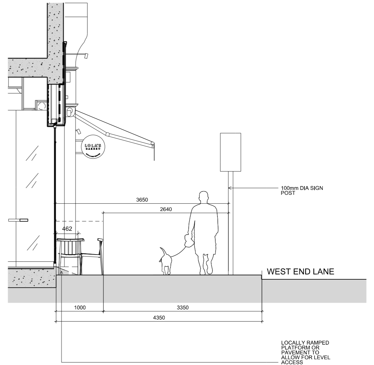
02 PROPOSED FRONT ELEVATION SECTION 1:50
