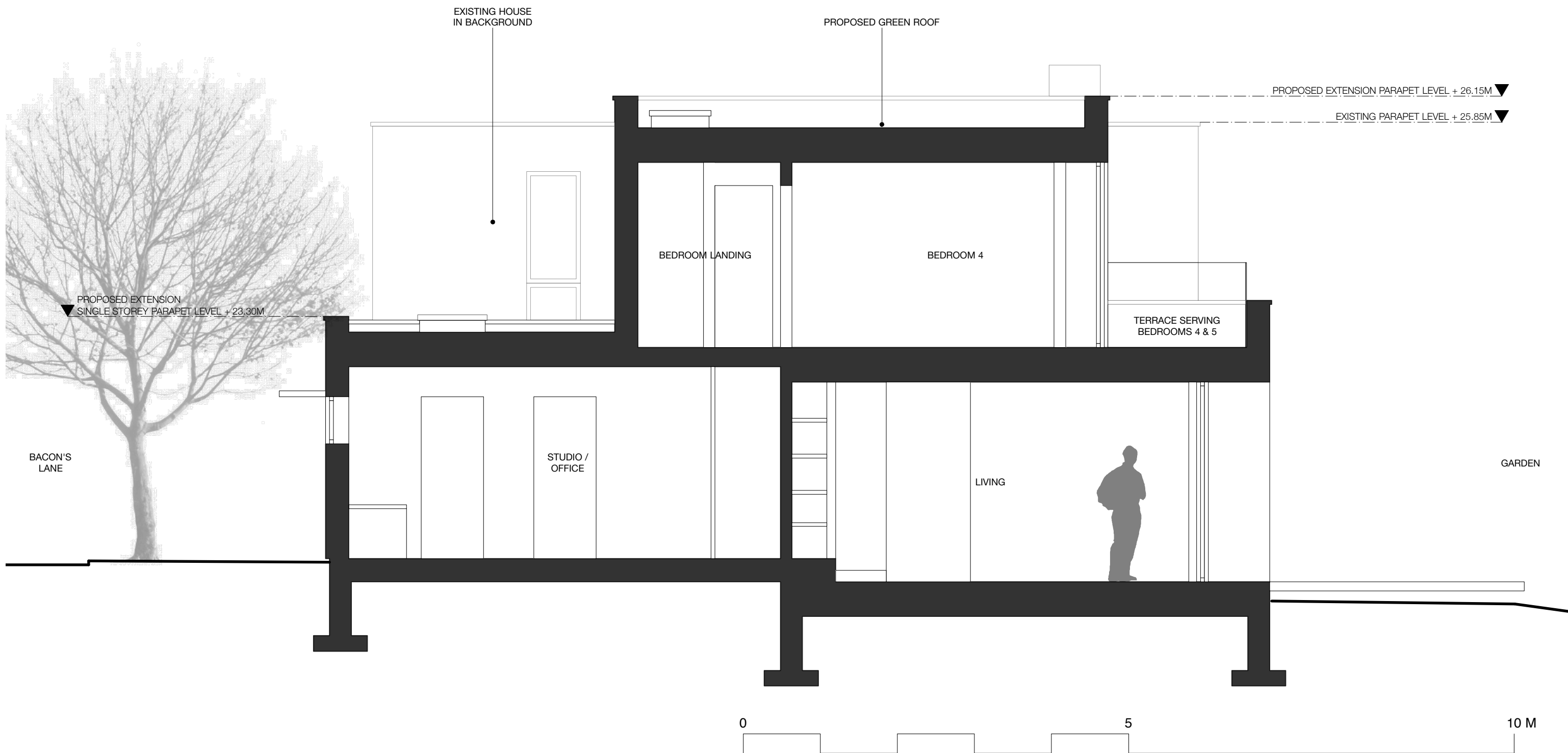
01 SECTION BB - PROPOSED 1:50
