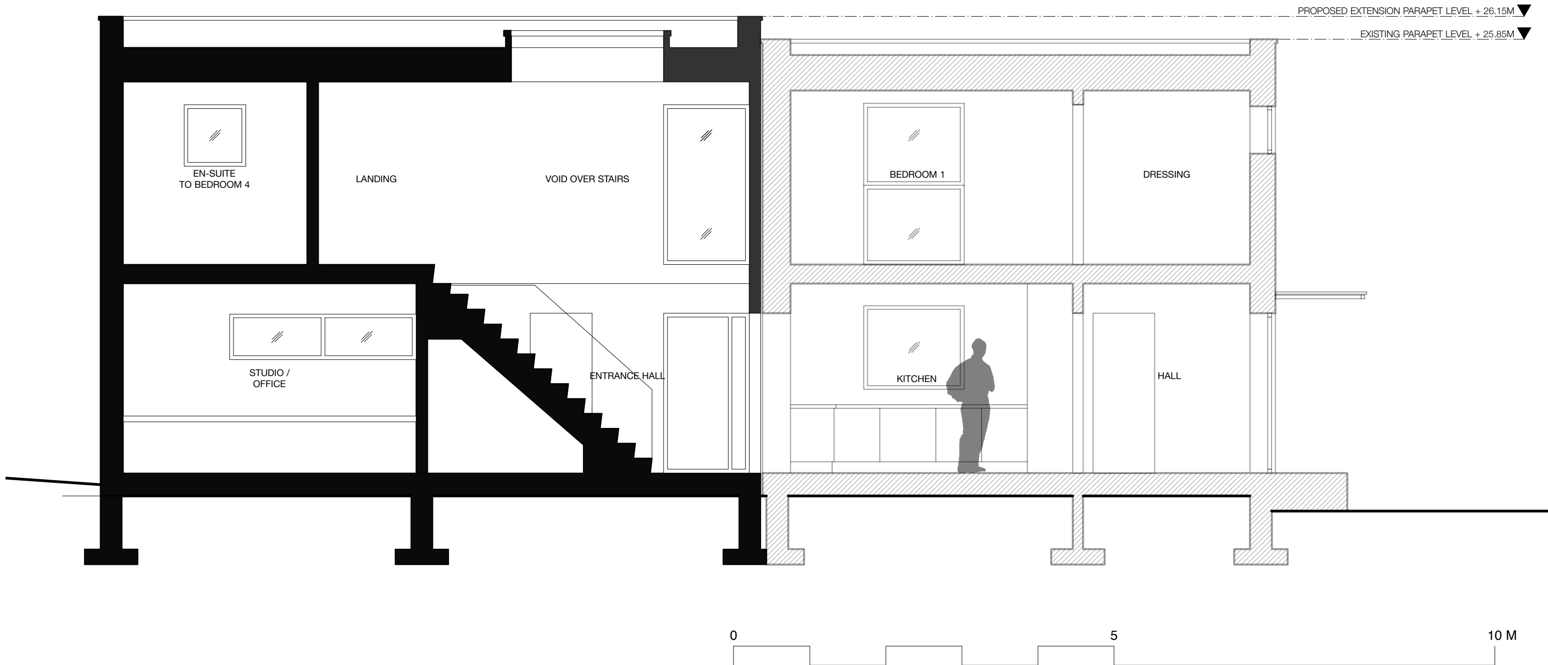
01 SECTION AA - PROPOSED & EXISTING 1:50
