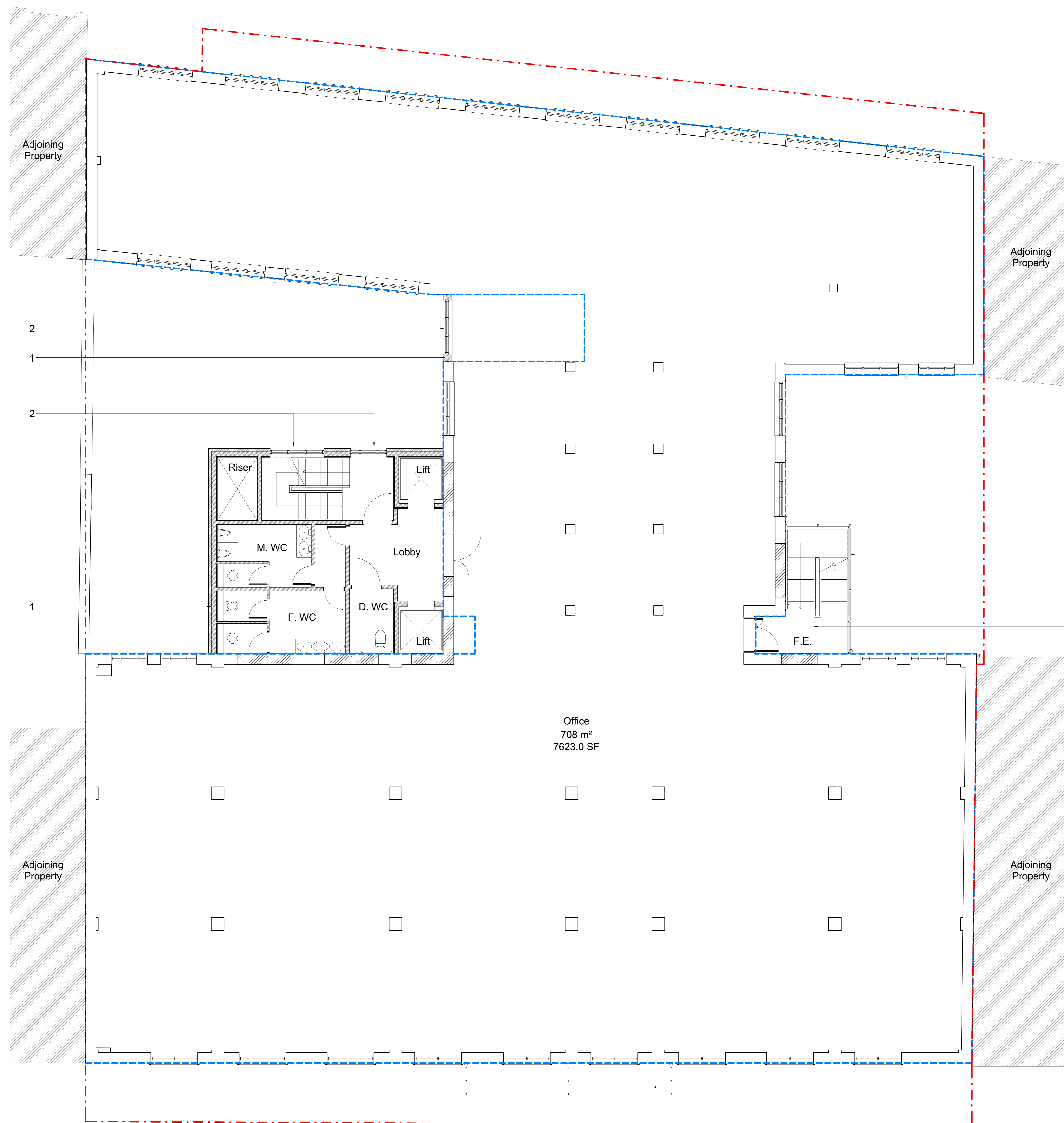
First Floor Plan as Proposed 1 : 50
