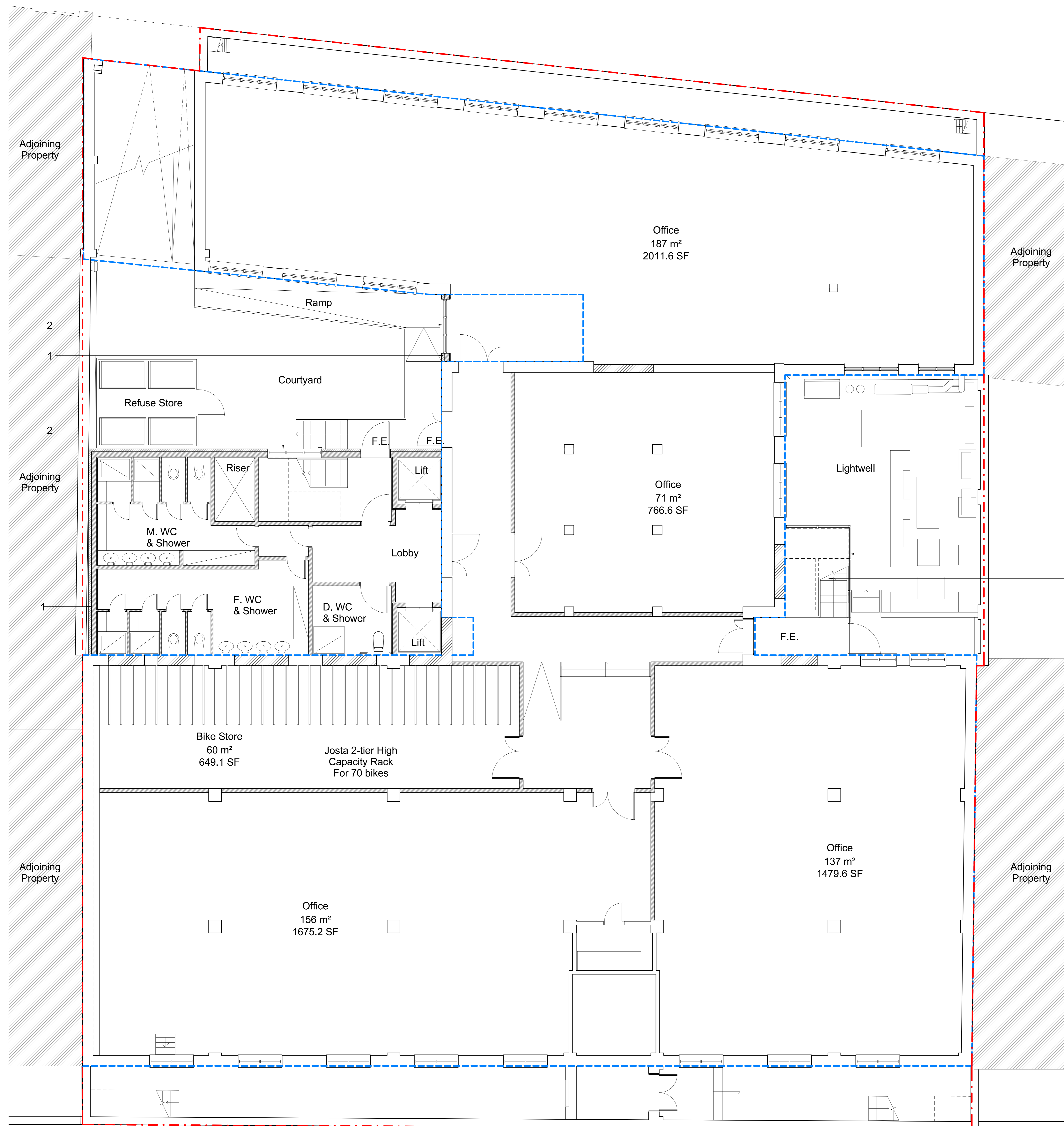
Lower Ground Floor Plan as Proposed 1 : 50
