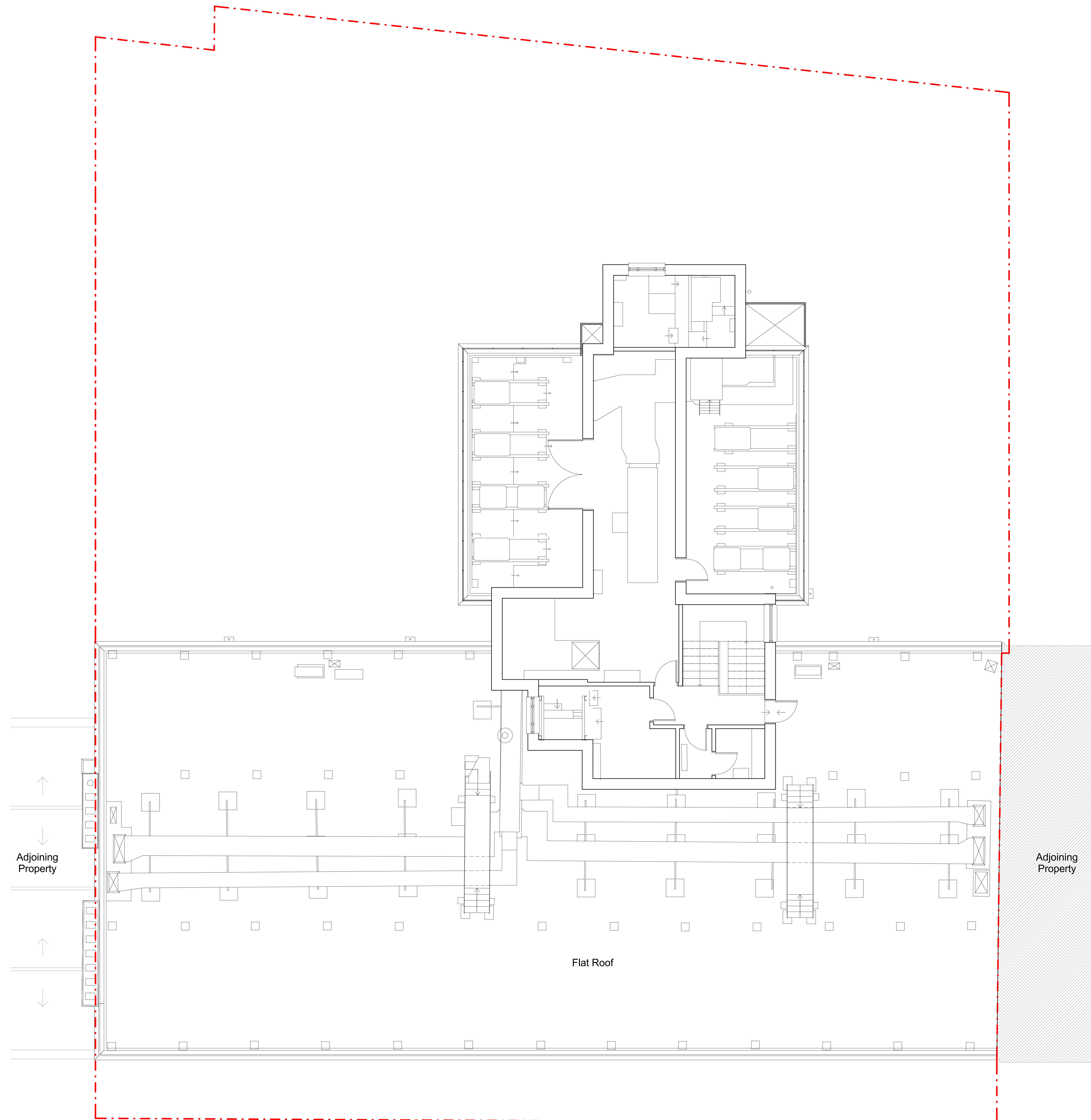
Fifth Floor Plan as Existing 1 : 50
