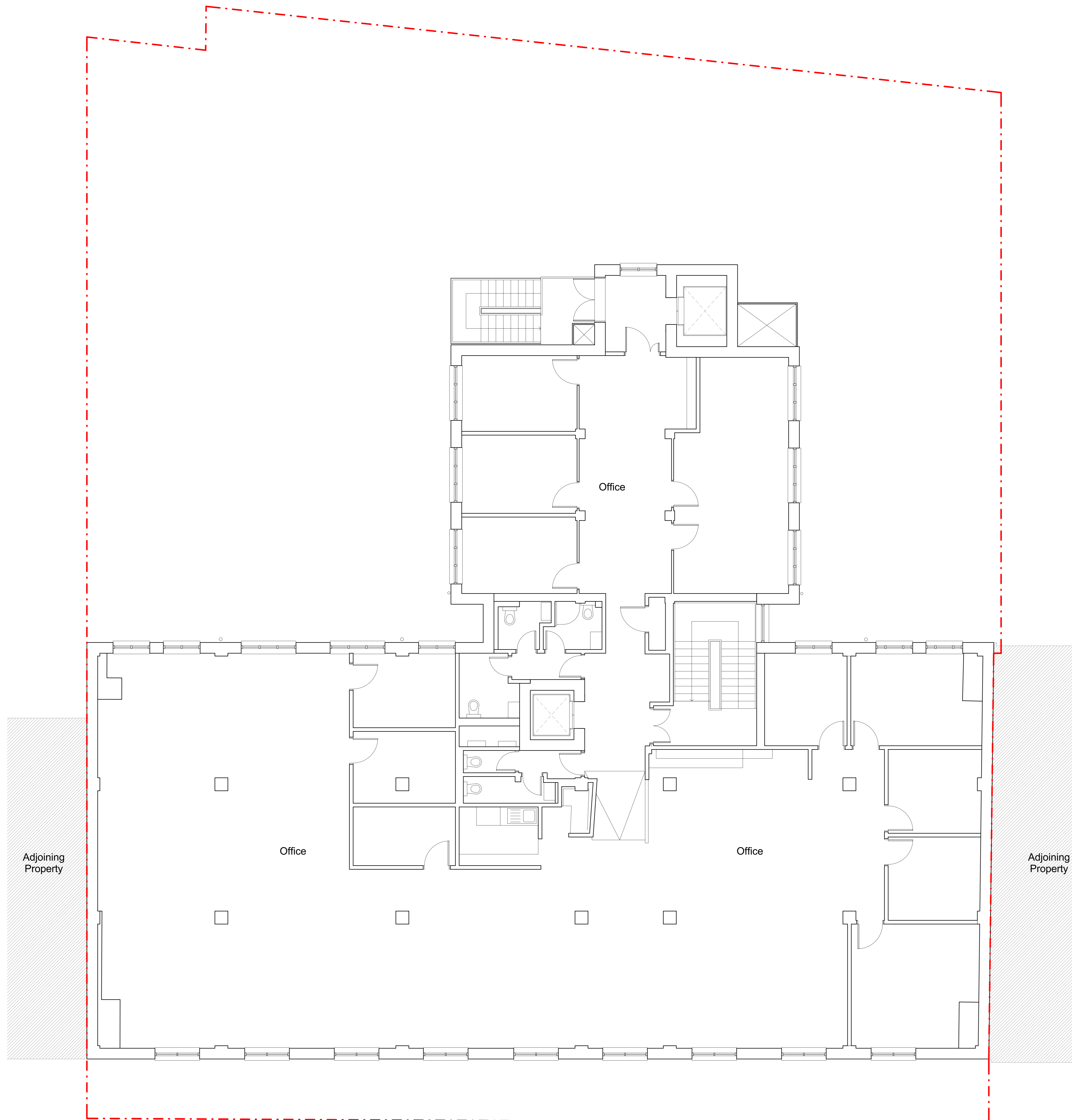
Fourth Floor Plan as Existing 1 : 50
