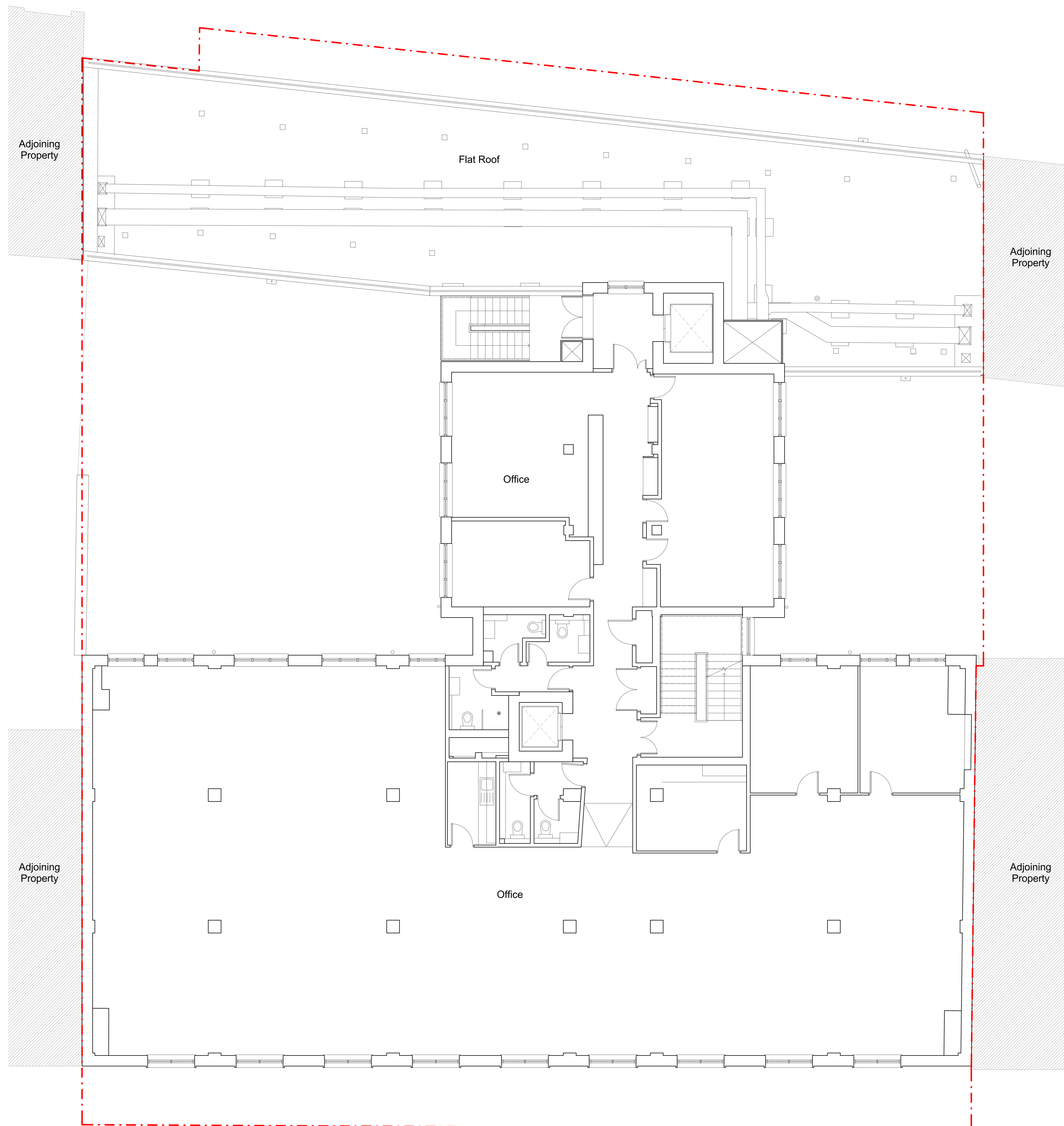
Second Floor Plan as Existing 1 : 50
