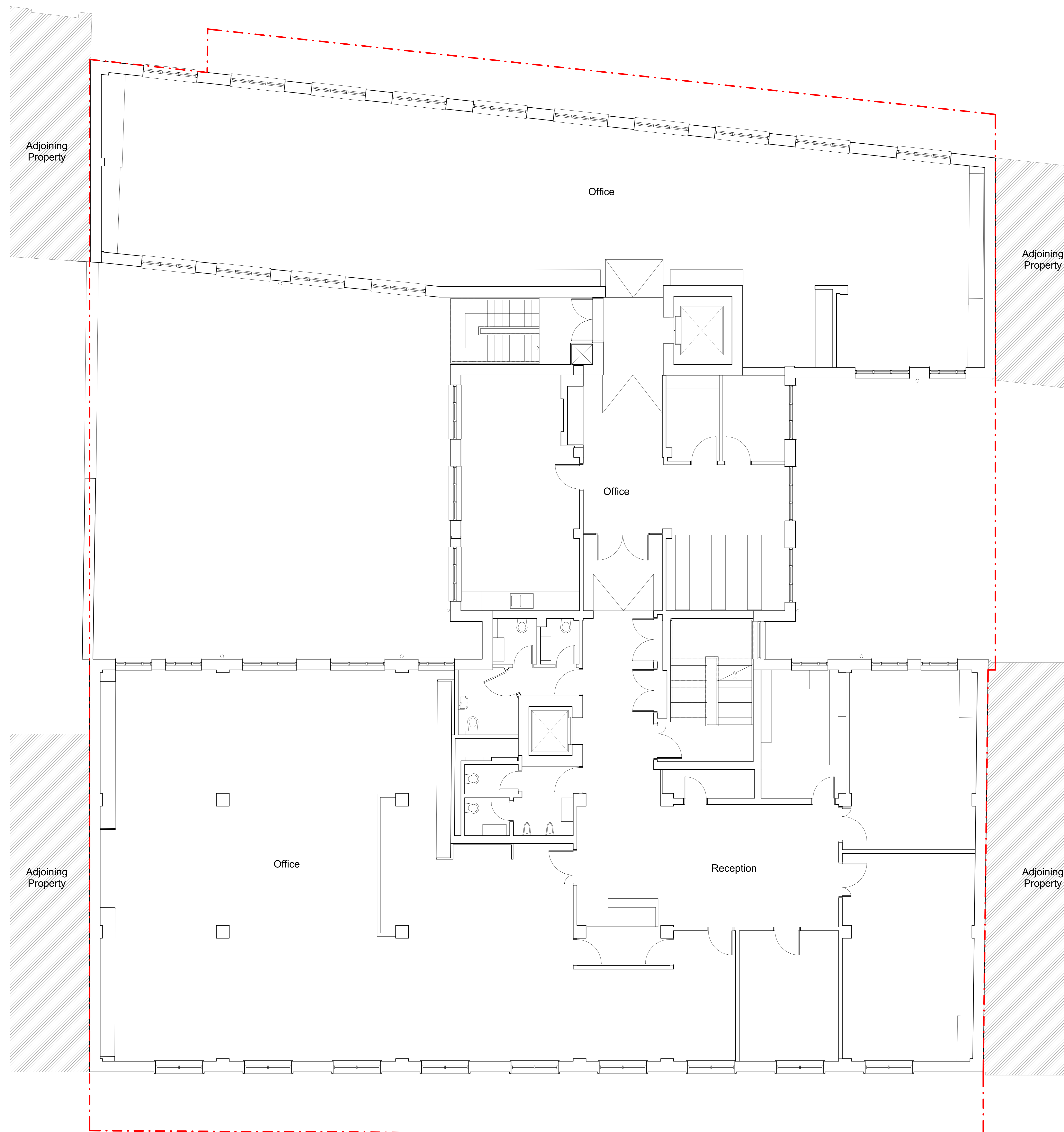
First Floor Plan as Existing 1 : 50
