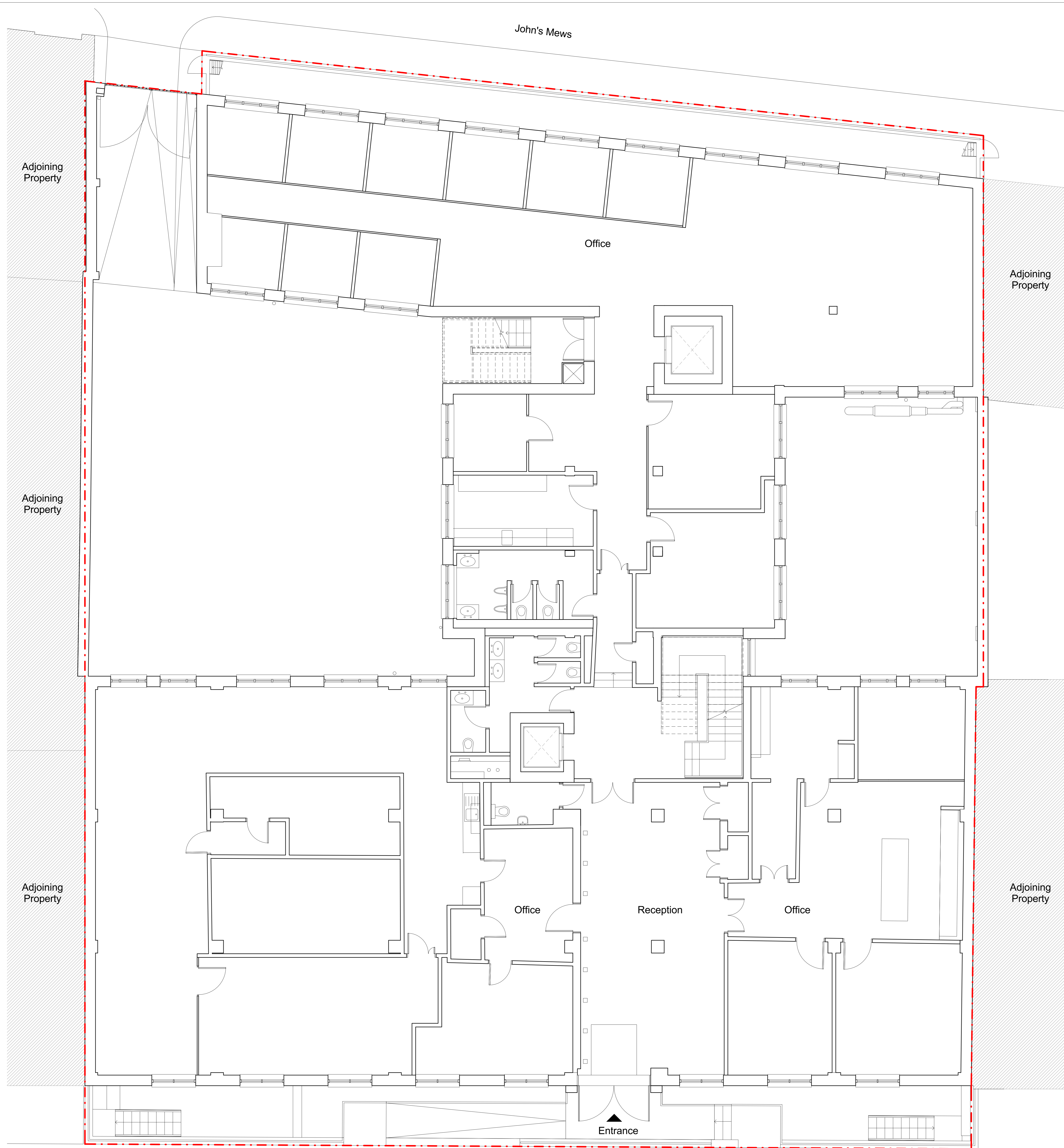
Ground Floor Plan as Existing 1:50
