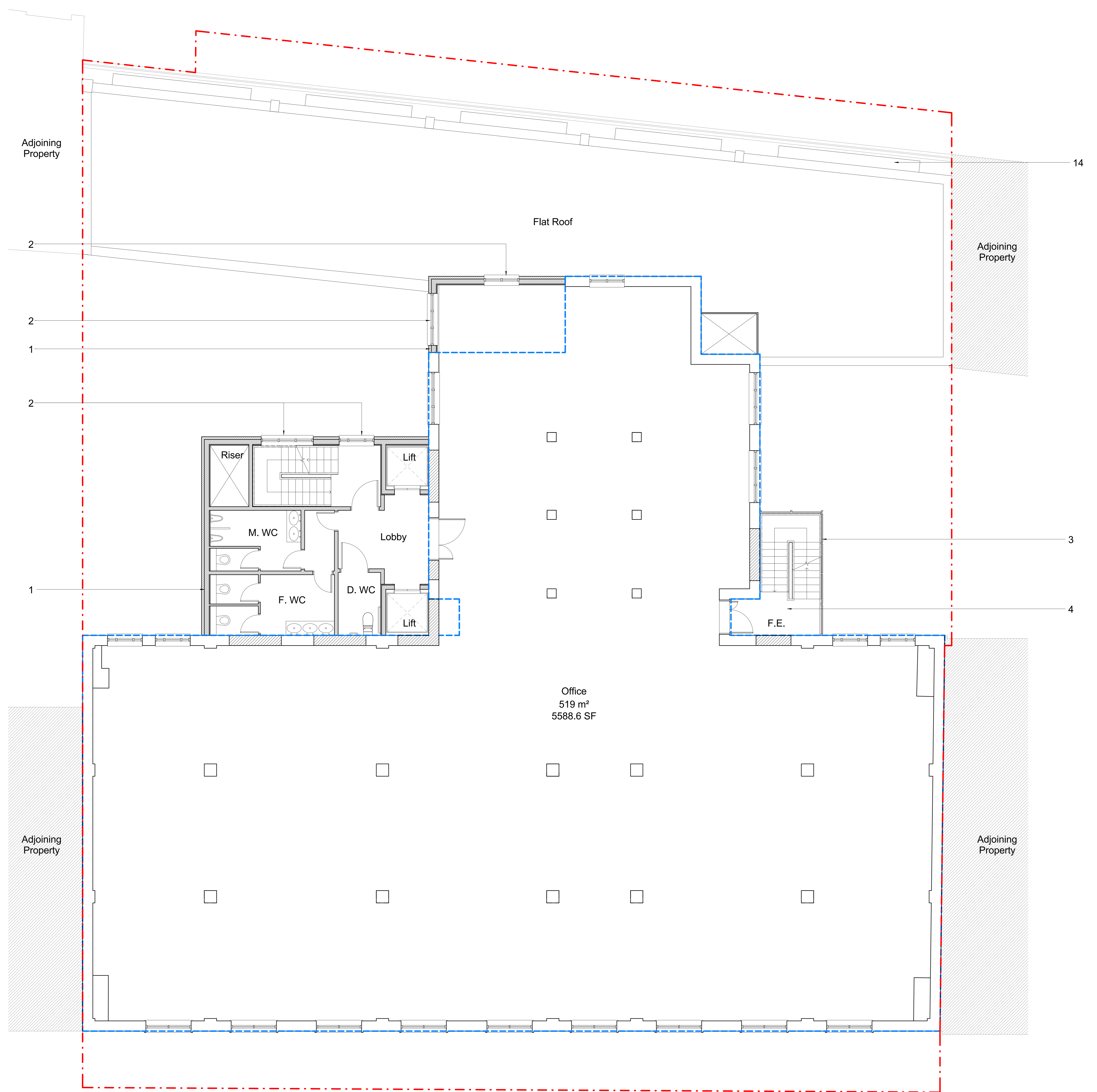
Third Floor Plan as Proposed 1 : 50
