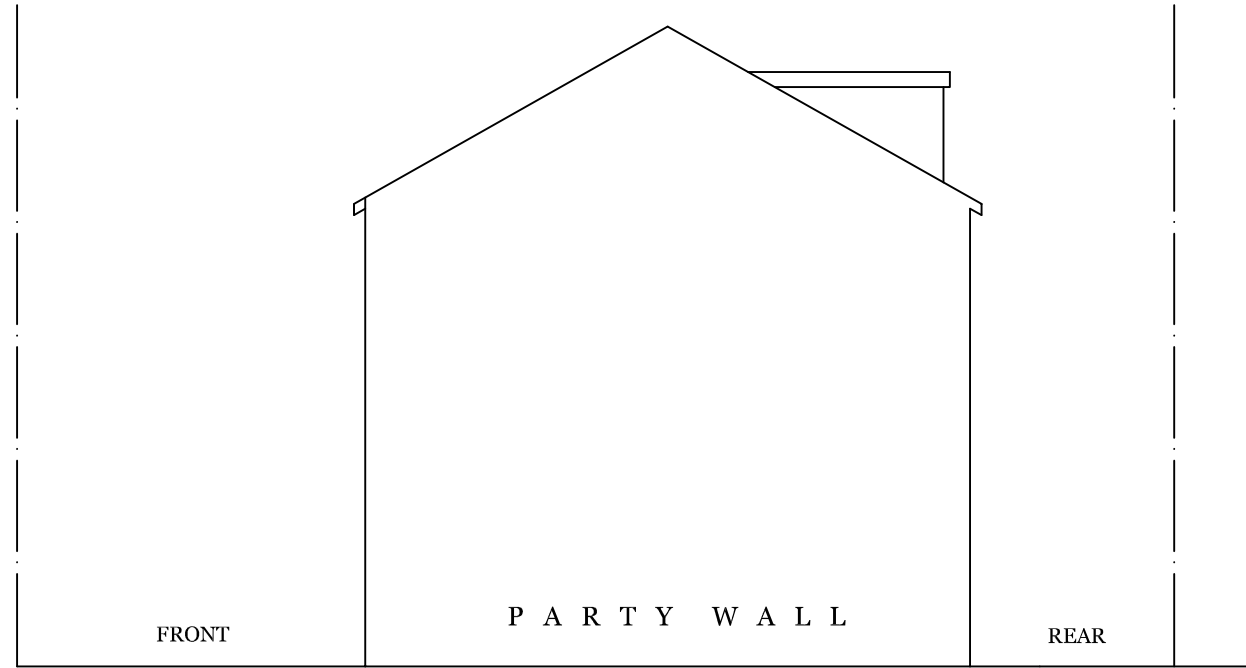
EXISTING & PROPOSED SIDE ELEVATION (UNCHANGED) 17 FAIRHAZEL GARDENS LONDON NW6
