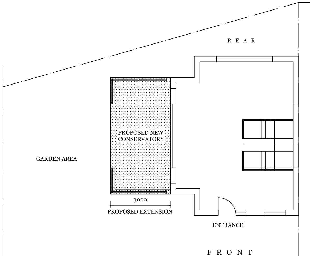
PROPOSED GROUND FLOOR 1:100 17 FAIRHAZEL GARDENS LONDON NW6
