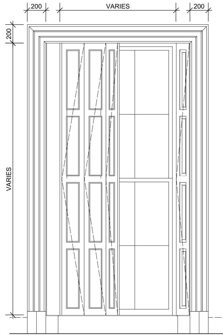
1 WINDOW SHUTTERS ELEVATION SCALE 1:25 PL-52
