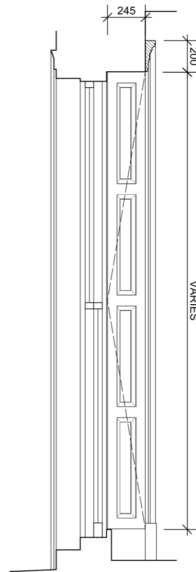
2 WINDOW SHUTTERS SECTION SCALE 1:25 PL-52
