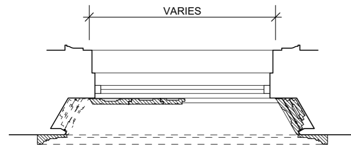
3 WINDOW SHUTTERS PLAN SCALE 1:25 PL-52
