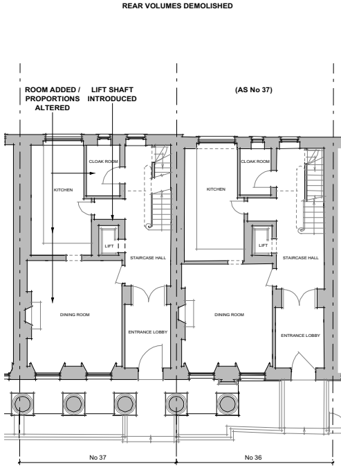
7 GROUND FLOOR PLAN YEAR : 1960's PL-32
