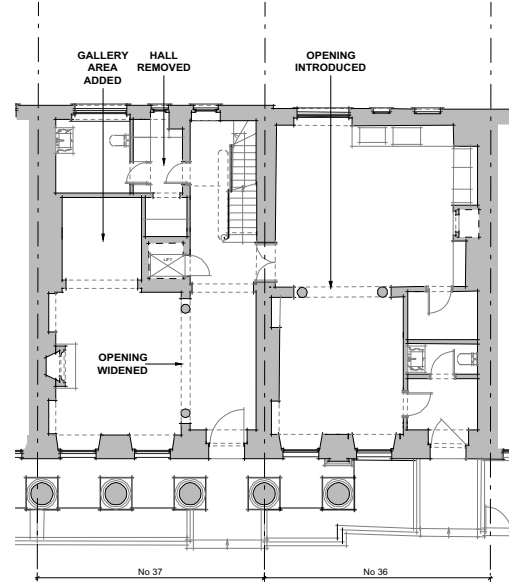
10 GROUND FLOOR PLAN PROPOSED PL-32
