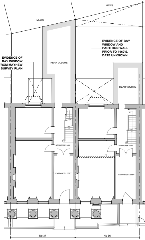
6 GROUND FLOOR PLAN ORIGINAL PL-32
