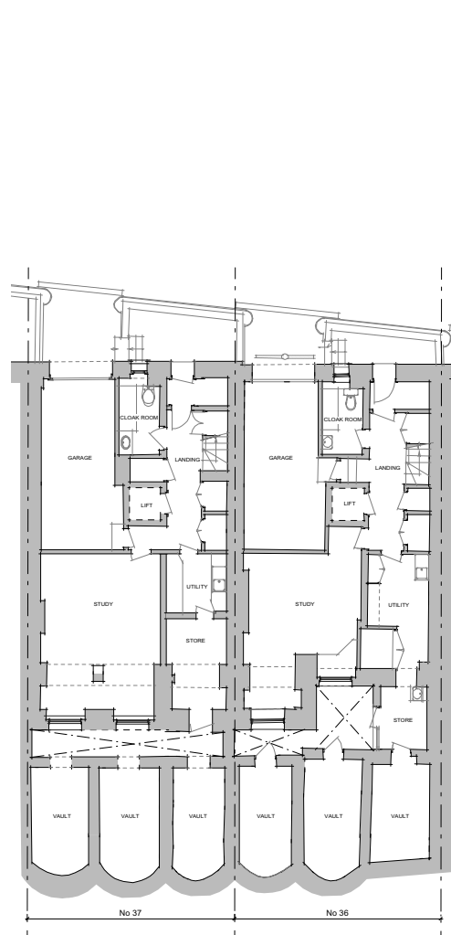
3 LOWER GROUND FLOOR PLAN YEAR : 2009 PL-32
