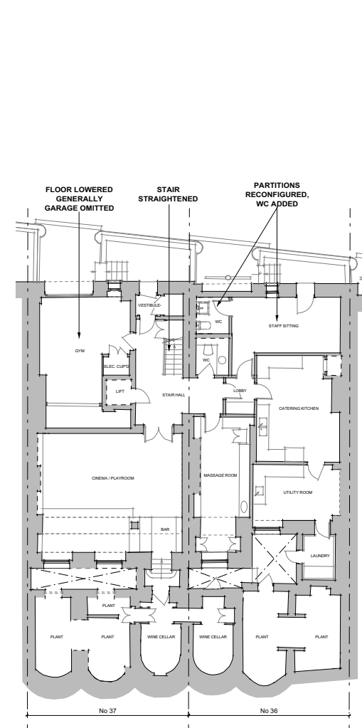
5 LOWER GROUND FLOOR PLAN PROPOSED PL-32
