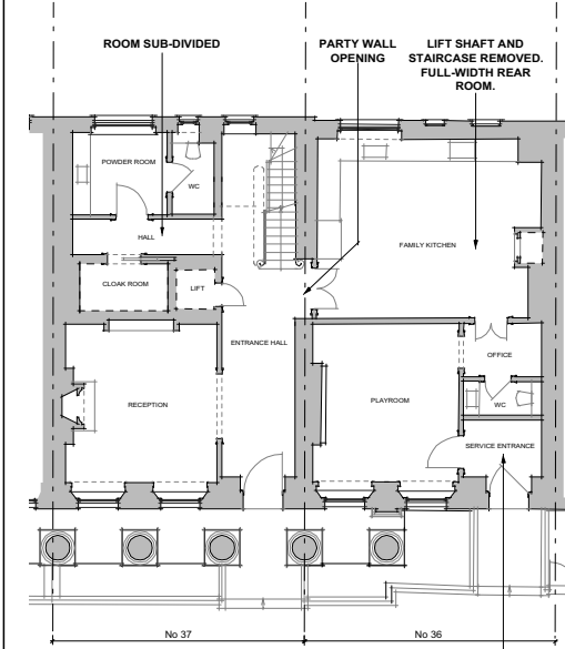
9 GROUND FLOOR PLAN YEAR : 2017 (EXISTING) PL-32
