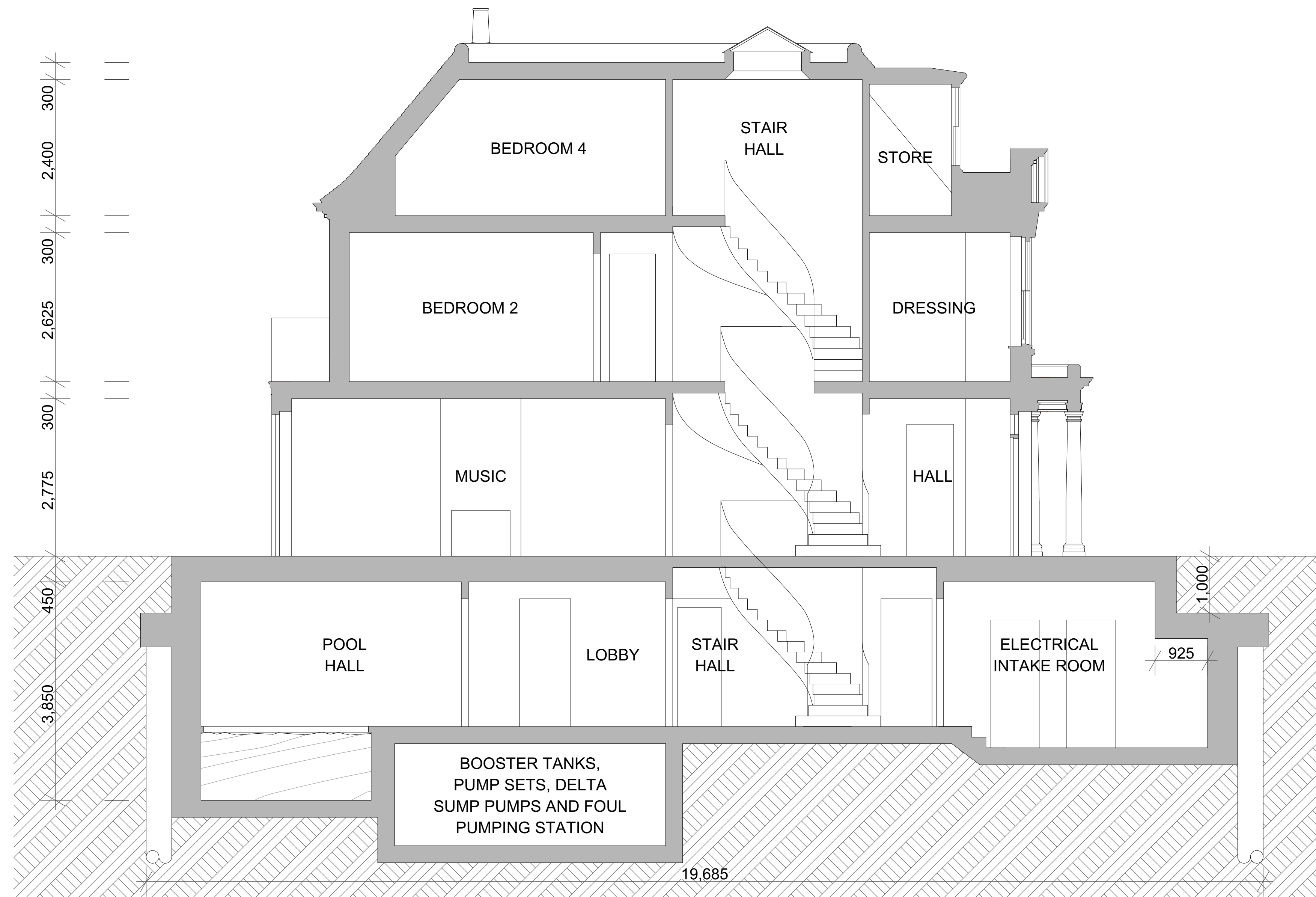
LONG SECTION
