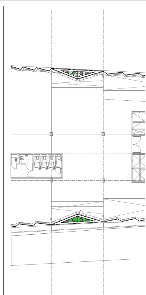
05 LEVEL 06 FLOOR PLAN 00011
