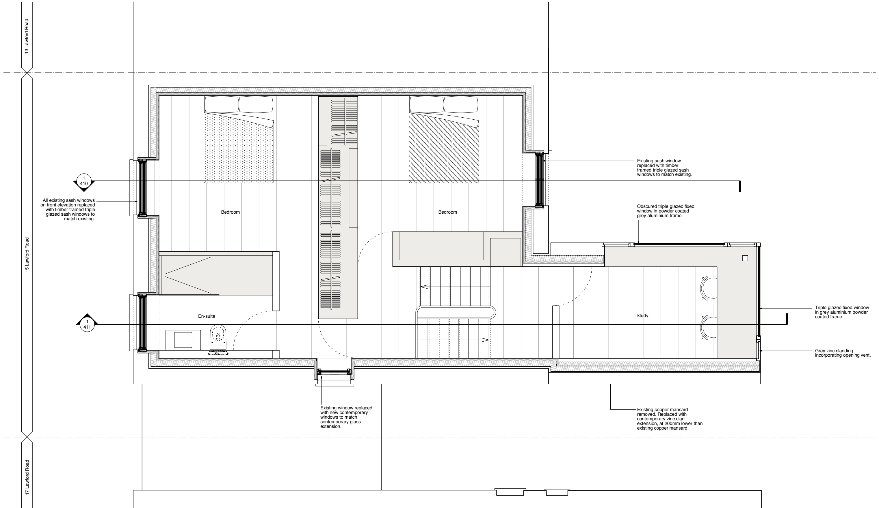
1 Proposed Second Floor Plan 1:50@A3
