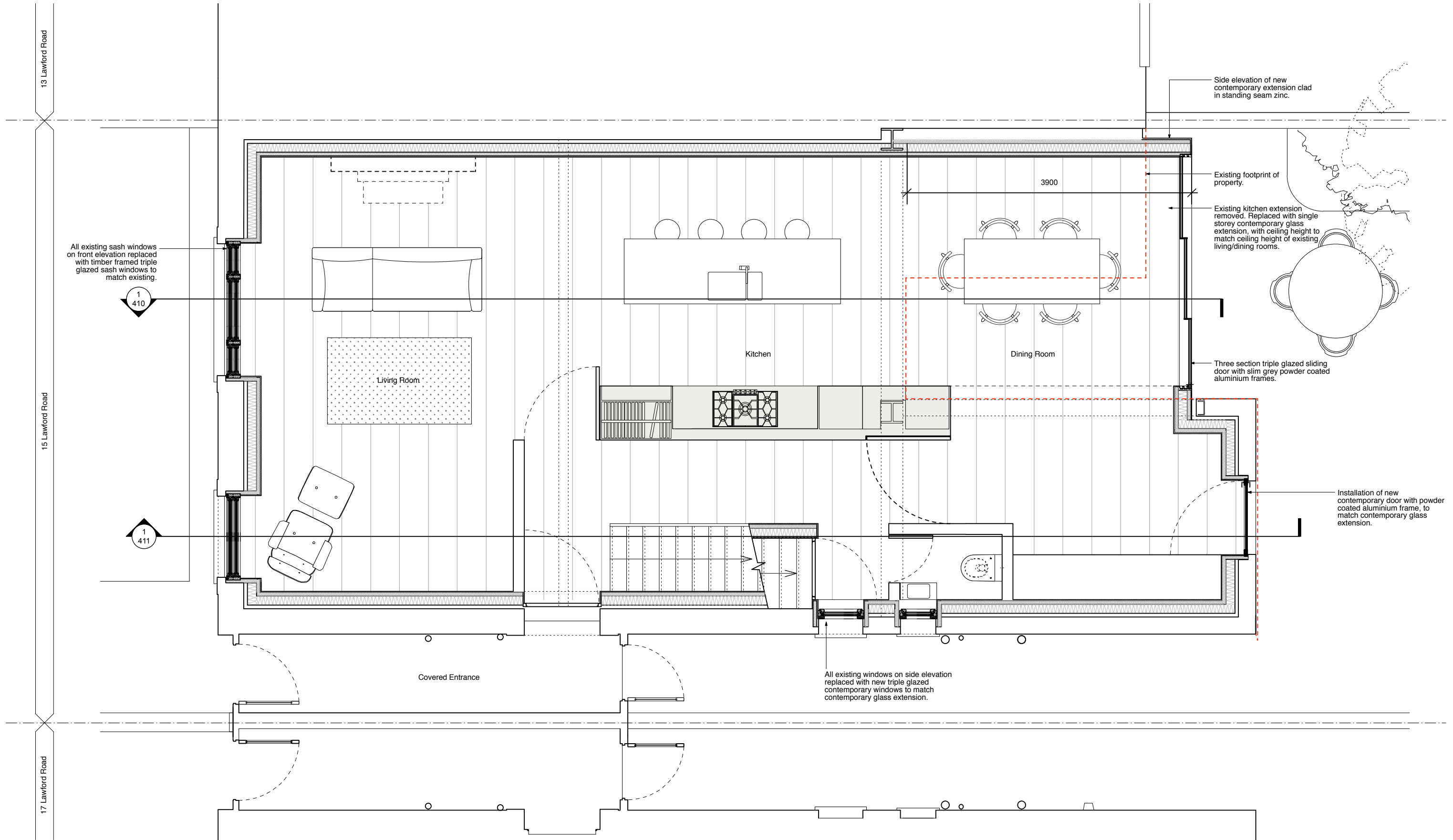
1 Proposed Ground Floor Plan 1:50@A3
