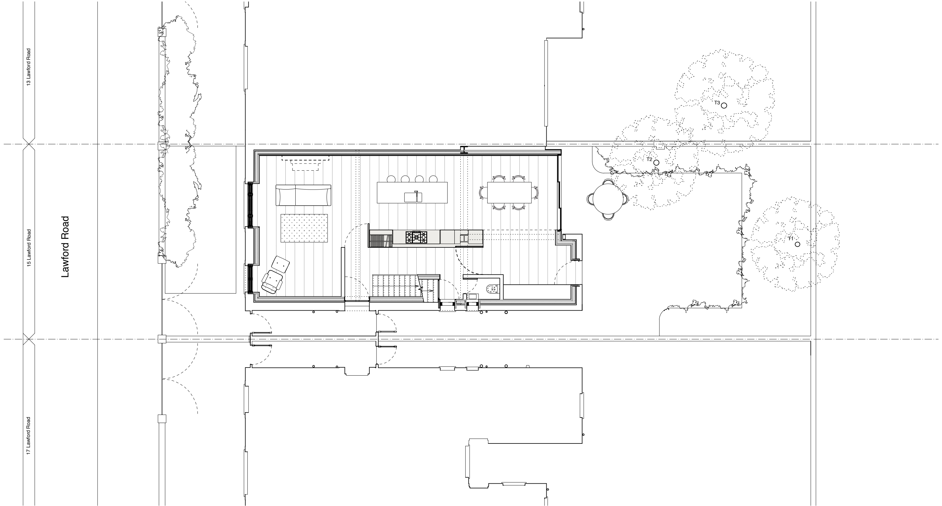
1 Proposed Site Plan 1:100@A3
